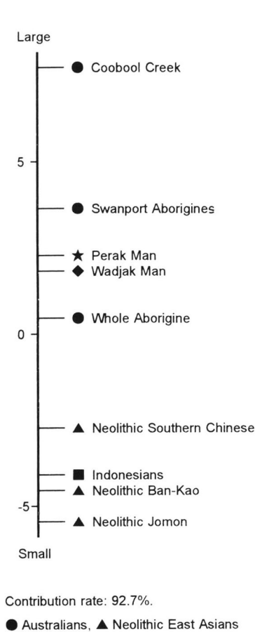
Fig. 2. One dimensional expression of MDS applied to the PENROSE's size distances based on the nine buccolingual crown diameters.
