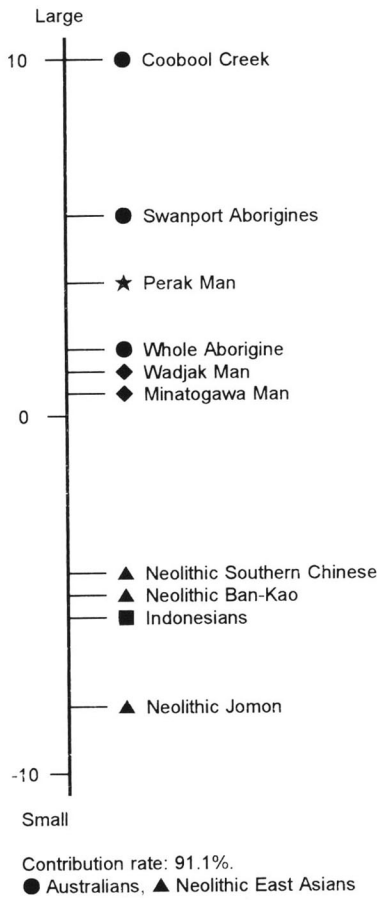
Fig. 3. One dimensional expression of MDS applied to the PENROSE's size distances based on the seven buccolingual crown diameters.
