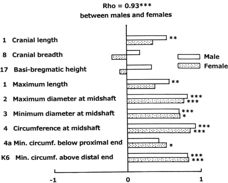
Fig. 2. Factor loadings on the first principal components obtained from the data sets of the neurocranium and fibula for males and females. For the numbers preceding measurement items, see the second footnote to Table 3.
