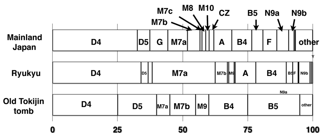
Fig. 2. Estimated frequencies of the mtDNA haplogroups in regional populations.
