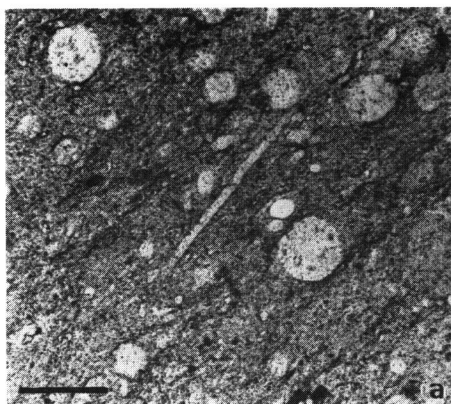
Fig. 1a. Cherty part showing well preserved radiolarian tests and sponge spicule (centre). Polarizer only. Bar: 0.1 mm
