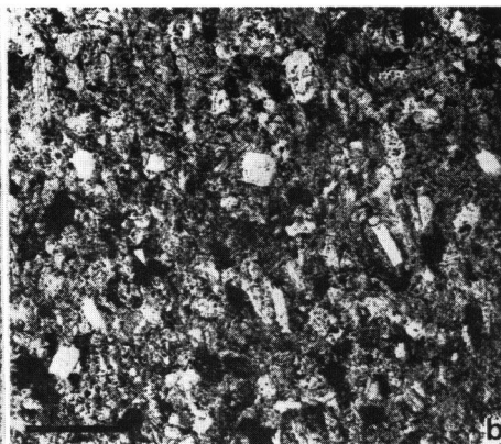
Fig. 1b. Sandy part showing ordinary sandstone texture. No organic remain is visible in the field, although the sandy part includes a quite few radiolarians and spicules. Polarizer only. Bar: 0.1 mm
