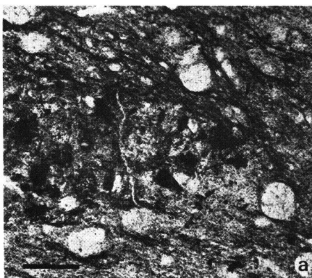
Fig. 2 a, b. Wavy and flowing structure of clayey matrix surrounding sandstone lumps in chert. The circular outlines of radiolaria are neither deformed nor distorted. Polarizer only. Bar: 0.1 mm
