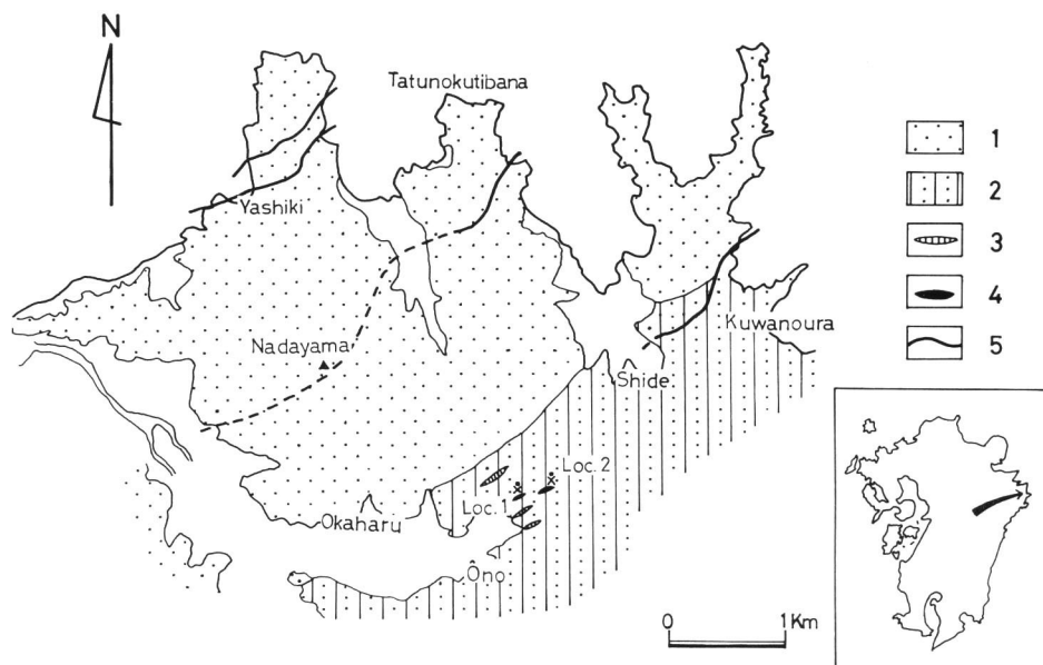
Fig. 1. Geological map (HASHIMOTO, 1962) around fossil localities.
