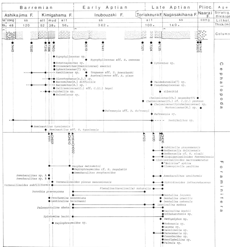
Text-fig. 2. Stratigraphic distribution of cephalopods and foraminifers in the Choshi section. Loose pebbles and blocks are shown in brackets. Read Miocene for Pliocene.
