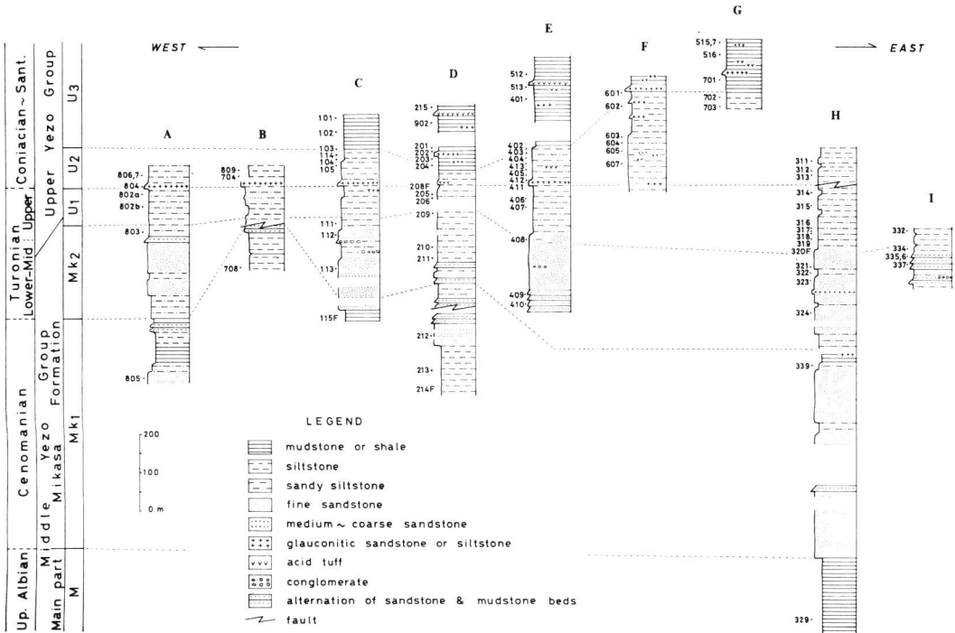
Fig. 4. The columnar sections in the Kamiichi-no-sawa area, Ikushumbetsu, central Hokkaido.
