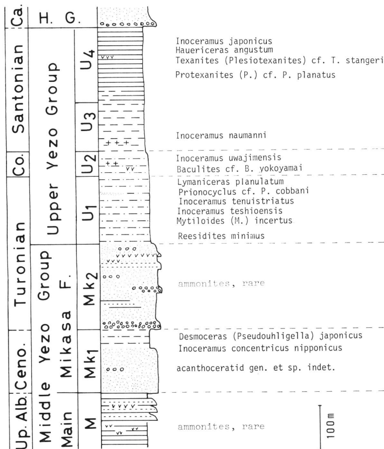
Fig. 9. The generalized columnar section of the Bibai area, central Hokkaido. Rock symbols are the same as in Fig. 10.
