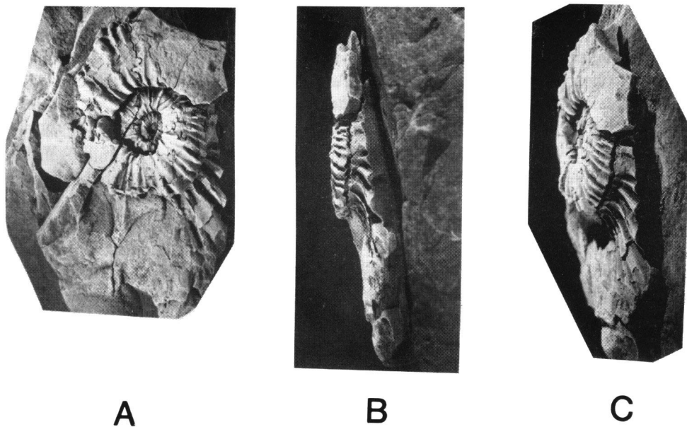
Text-fig. 2. Acanthohoplites reesei (ANDERSON), from the Upper Member of the Sebayashi Formation, Upper Aptian. GPM-GIII1h30 (I. TAMURA coll.). Lateral (A), ventral (B) and diagonal (C) views, \times 1.2 .
