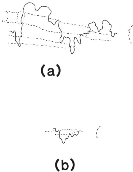
Text-fig. 3. Acanthohoplites reesidei (ANDERSON). External suture-line of the Sanchu specimen, GPM-GIIIh30, at whorl-height of ca 4.4 mm (a) and 3.5 mm (b).
