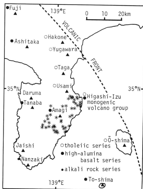
Fig. 1. Quaternary volcanoes in Izu Peninsula. Asterisks are vents of Higashi-Izu monogenic volcano group (HAMURO, 1985).
