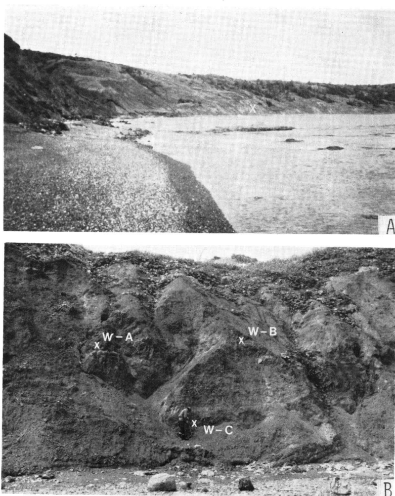
Fig. 1. The strata of the Middle Yezo Group exposed along the coastal cliff at Chenaibo in the Wakkanai area (A) and the sample positions (B).
