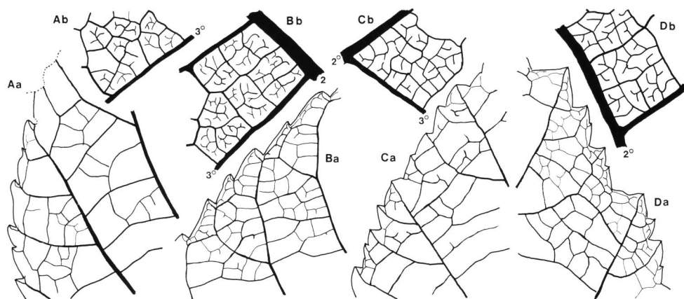
Fig. 3. The marginal venation features and areoles of Paleogene leaves of Alnus and Corylus and their related extant species. 2^\circ and 3^\circ in each figure indicate the secondary and tertiary veins, respectively. Aa, b, Alnus kushiroensis TANAI, NSM-PP 10560, Aa \times 2.5 , Ab \times 12.5 ; Ba, b, Alnus subcordata C. A. MEY, NSM Paleobot. Ref. Coll. T-1812, Ba \times 3 , Bb \times 12.5 ; Ca, b, Corylus palaeomaximowicziana (ENDO) TANAI, NSM 10469 (=NSM-PP 1785), Ca \times 2.5 , Cb \times 12.5 ; Da, b, Corylus chinensis FRANCH, NSM Paleobot. Ref. Coll. T-1886, Da \times 2.5 , Db \times 12.5 .
