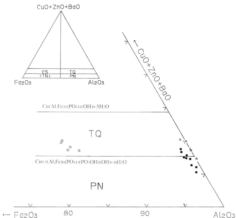
Fig. 2. Chemical compositions of turquoise and planerite plotted on (\text{CuO}+\text{ZnO}+\text{BaO})-\text{Al}_2\text{O}_3-\text{Fe}_2\text{O}_3 diagram.
