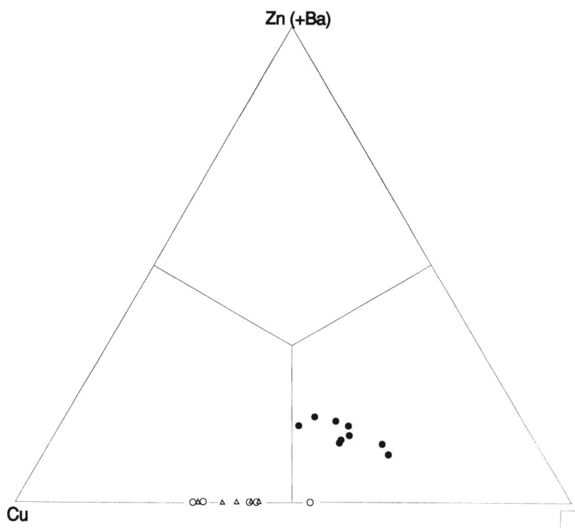
Fig. 3. Mole ratio of Cu, Zn (+Ba), and vacancy in turquoise and planerite. Note the higher ZnO contents in planerite.
