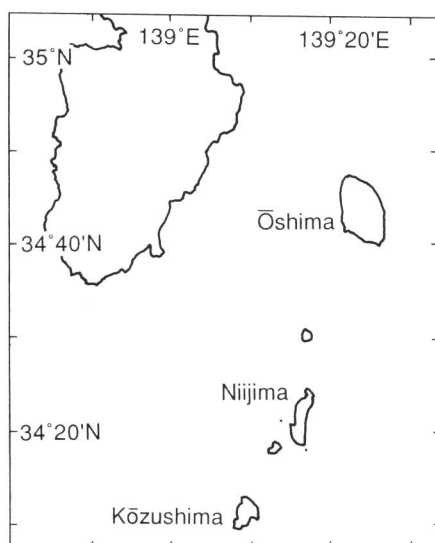
Fig. 1. Index map of Ōshima, Niiijima and Kōzushima.
