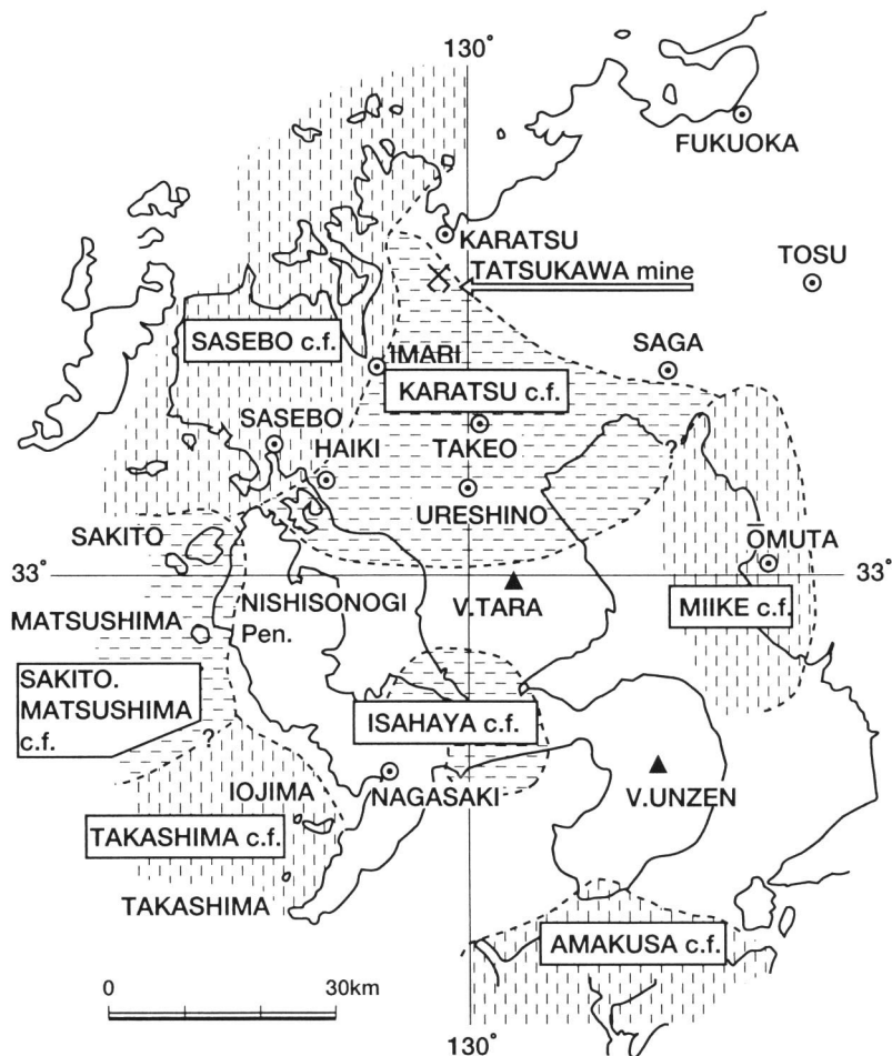
Fig. 1. Distribution of Tertiary coal-fields in northwestern Kyushu, Japan. c.f., coal-field; V., volcano; Pen., Peninsula.
