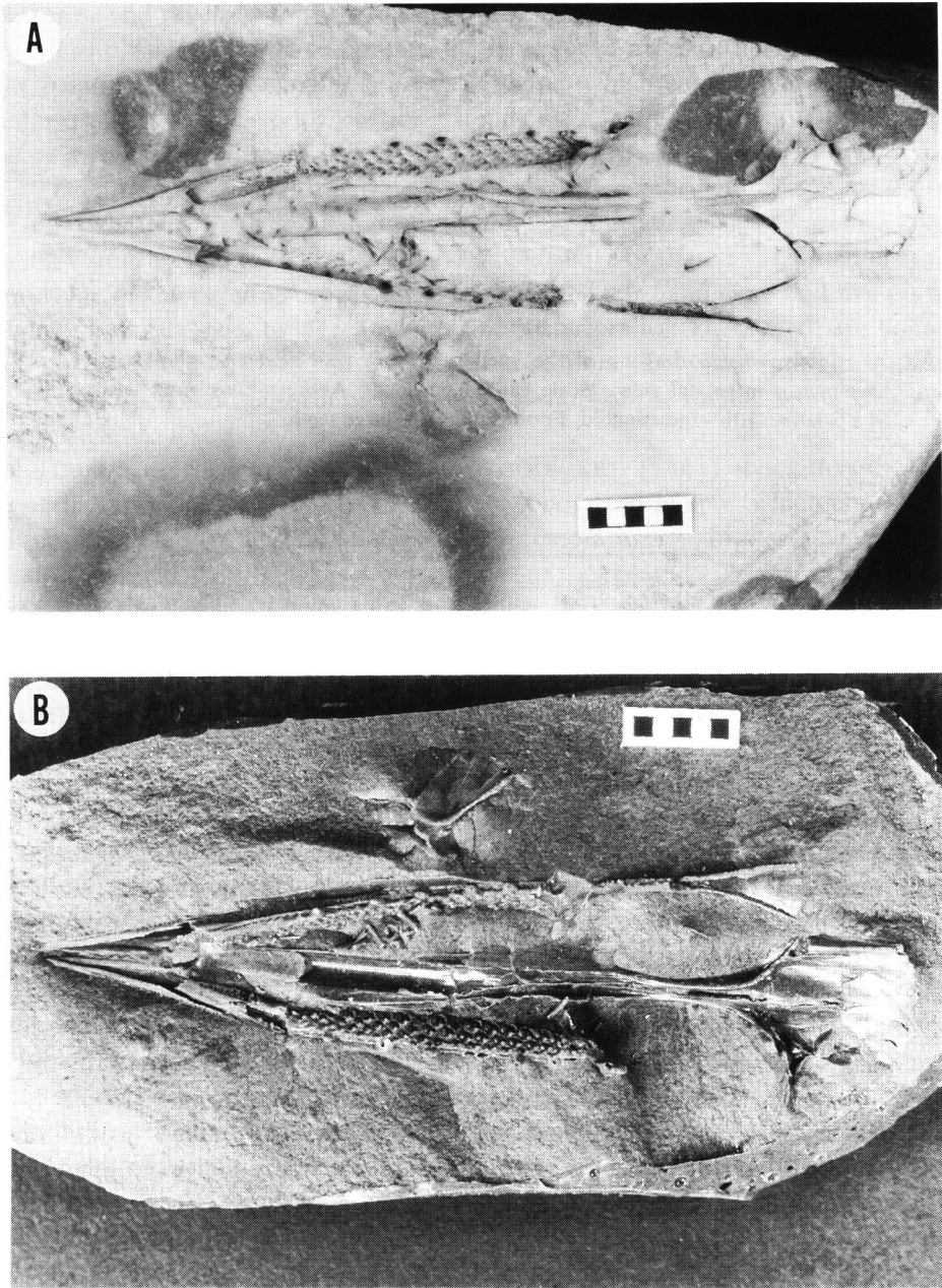
Fig. 3. A, photograph of the flint nodule containing the specimen of Dercetis elongatus in the private collection of Mr J. BURTONSHAW; B, photograph of the latex peel of the above specimen (BRSUG 24215). Both specimens show a palatal view. Scale bar in both photographs is 1 cm.
