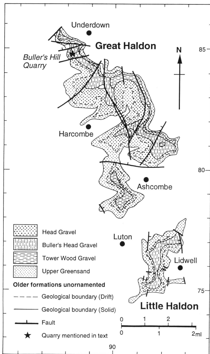
Fig. 2. Detailed geological map of the Haldon Hills area, Devon, England. Numbers around edge of map are Ordnance Survey Grid Reference numbers. Map adapted from EDWARDS and FRESHNEY (1982).
