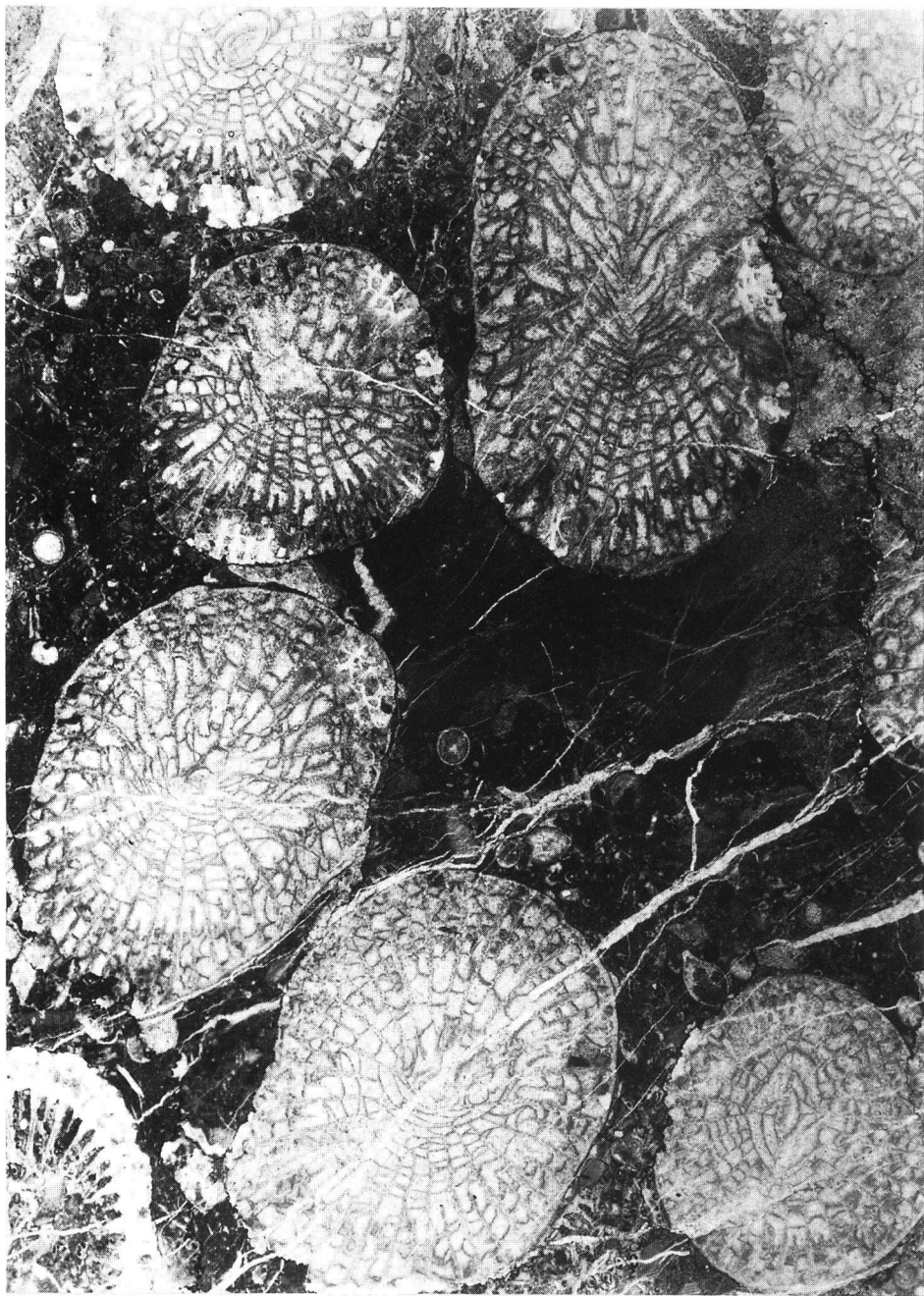
Fig. 3. Lithostroton ( Siphonodendron ) kamiyai Yamagiwa and Niko n. sp., holotype, NSM PA14340, transverse section, \times 5.0 .
