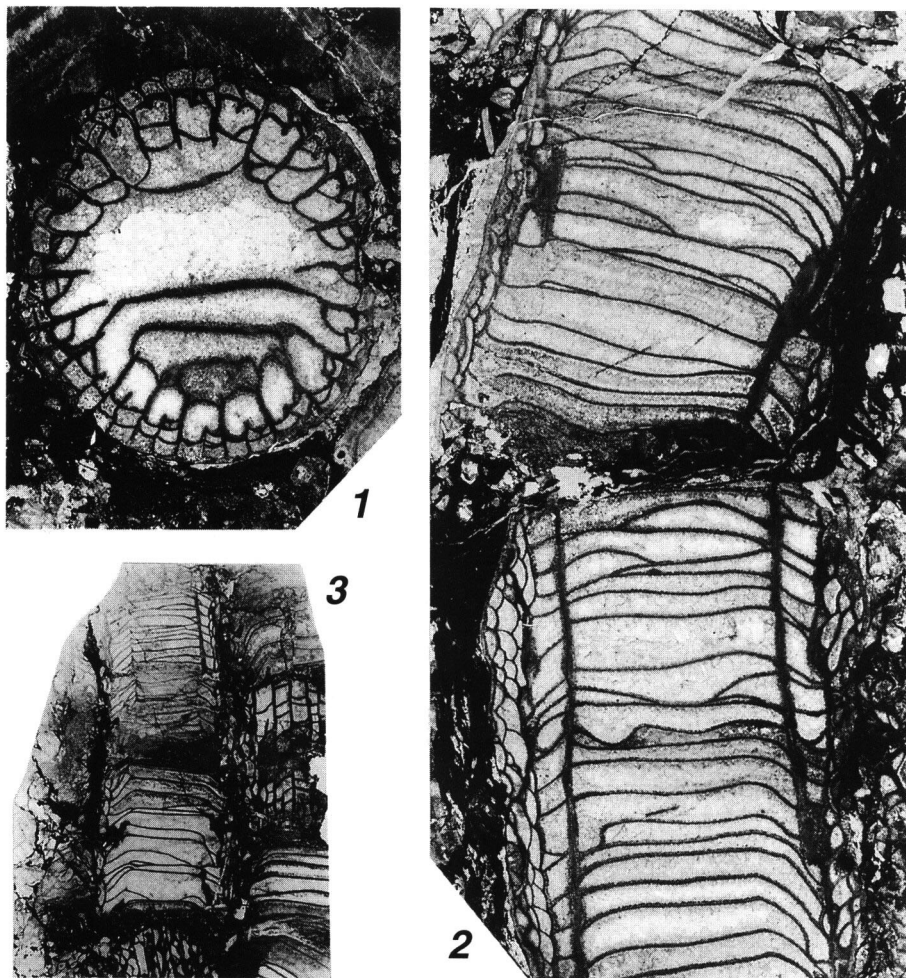
Fig. 5. Diphyphyllum sp. indet., NSM PA14345. 1. Transverse section, \times 5.0 ; 2, 3. Longitudinal sections, \times 5.0 and \times 2.1 , respectively.
