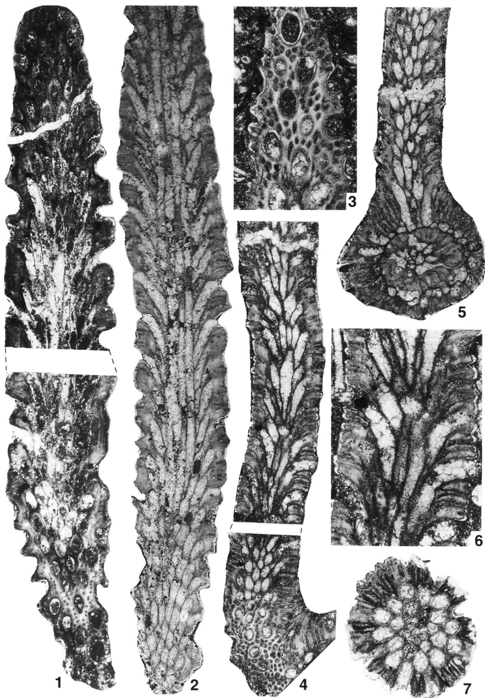
Fig. 8. 1, 2, Ascopora peruana n. sp., \times 20 , NSM PA-14219 and 14249b, respectively. 3–7, Pamirella andensis n. sp., 4, 5, \times 20 , NSM PA-14144f (holotype) and 14147c, respectively. 3, 6, enlarged parts of 4, in \times 40 ; 7, \times 40 , NSM PA-14144g.
