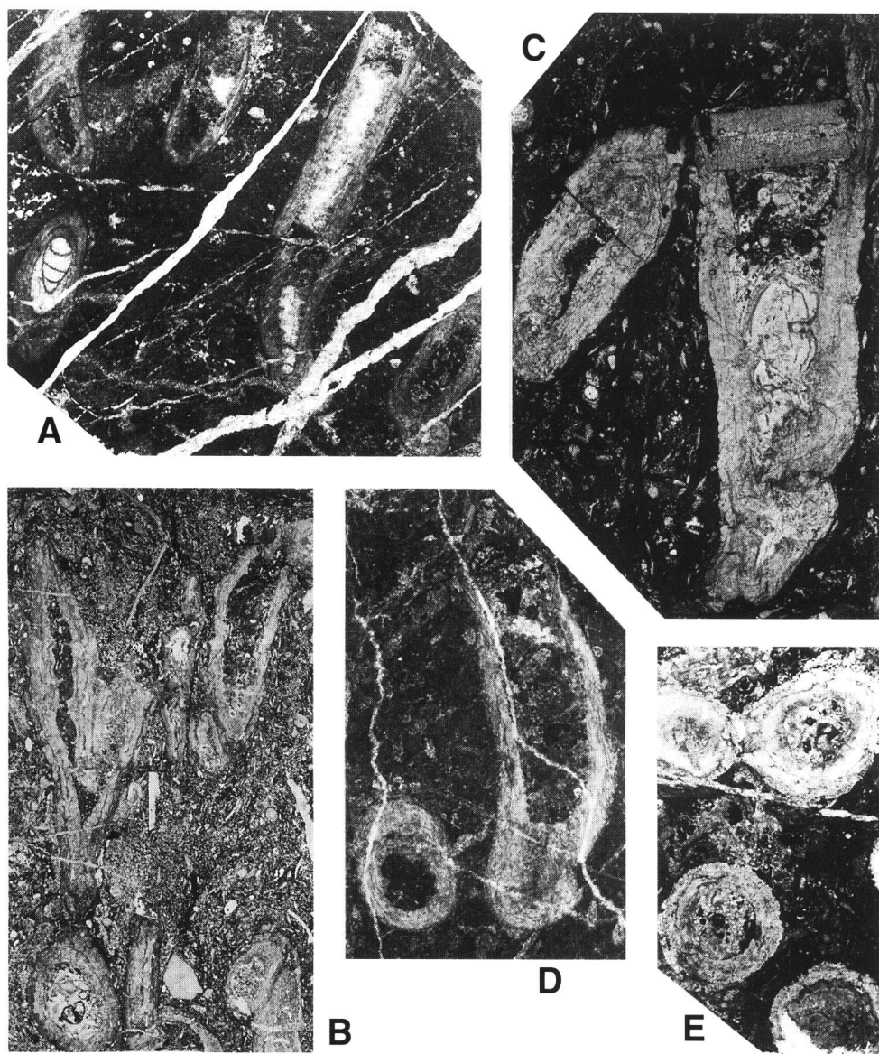
Fig. 4. A, D, Multithecopora? sp. indet. 1, NSM PA14379, thin sections, A, longitudinal section, \times 5 , D, longitudinal and transverse sections, \times 10 . B, C, Remesia? sp. indet., NSM PA14371, thin sections, B, longitudinal and transverse sections, \times 5 , C, longitudinal section, \times 10 . E, Cladochonus hamadai Igo and Adachi, NSM PA14373, thin transverse section, parallel to substrate, \times 10 .
