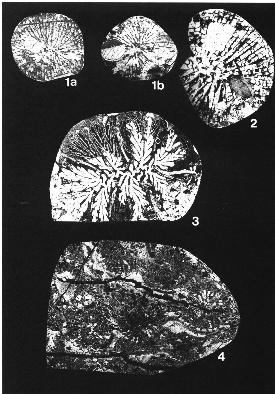
Fig. 4. 1–2, Montlivaltia sp. cfr. M. Xainzaens Liau. 1a–b. Transverse sections, \times 3.0 (NSM PA14263); 2. Transverse section, \times 3.0 (NSM PA14264). 3, Trochoidomeandra sp. indet. Transverse section, \times 3.0 (NSM PA14265). 4, Placocoenia ohinataensis Eguchi. Transverse section, \times 3.0 (NSM PA14266).
