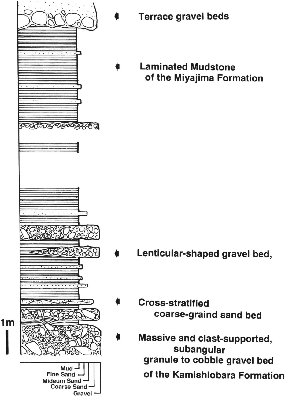
Fig. 6. Columnar section showing interfingering of the Kamishiobara and Miyajima formations at Loc. 1109.
