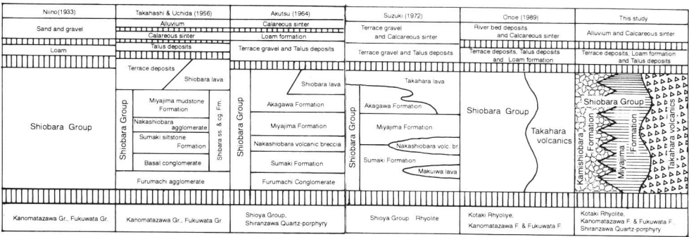
Fig. 2. Comparison of the lithostratigraphic divisions of the Shiobara Group.
