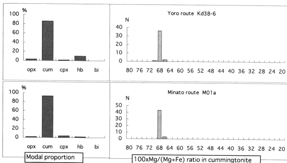
Fig. 3. Comparison of modal proportion and chemical composition of cummingtonite in “Kd38” tuff from the Yoro route and M01a tuff from the Minato route. Abbreviation of minerals are in Table 1.
