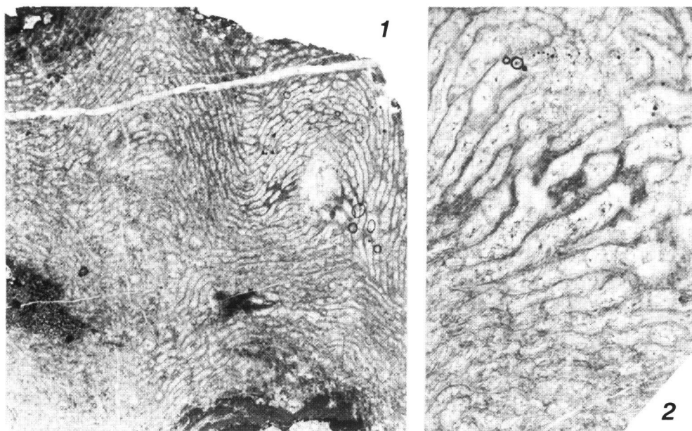
Fig. 4. Subalveolites ordinarius Kim, NSM PA14975, thin sections. 1, longitudinal section of corallum, showing ridge-like projections, \times 5 . 2, oblique sections of corallites, showing thickened intercorallite walls, \times 14 .
