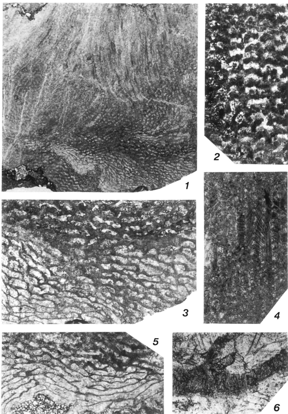
Fig. 6. Gionyamapora kambei gen. et sp. nov., holotype, NSM PA15001, thin sections. 1, longitudinal section of corallum, \times 5 . 2, transverse sections of proximal corallites, note intracolony columns, \times 14 . 3, oblique to transverse sections of proximal corallites, \times 14 . 4, longitudinal sections of distal corallites, \times 14 . 5, longitudinal sections of most proximal corallites, \times 14 . 6, partial enlargement to show intercorallite wall structure, \times 100 .
