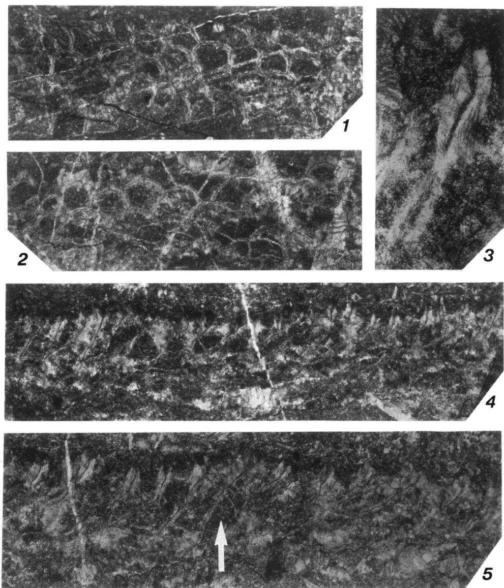
Fig. 9. Planocoenites oishinouchiensis sp. nov., thin sections. 1, paratype, NSM PA14660, transverse sections of corallites, \times 10 . 2–5, holotype, NSM PA14662. 2, transverse sections of corallites, \times 10 . 3, partial enlargement to show intercorallite wall structure, \times 50 . 4, longitudinal sections of corallites, \times 10 . 5, longitudinal sections of corallites, arrow indicates tabula, \times 14 .
