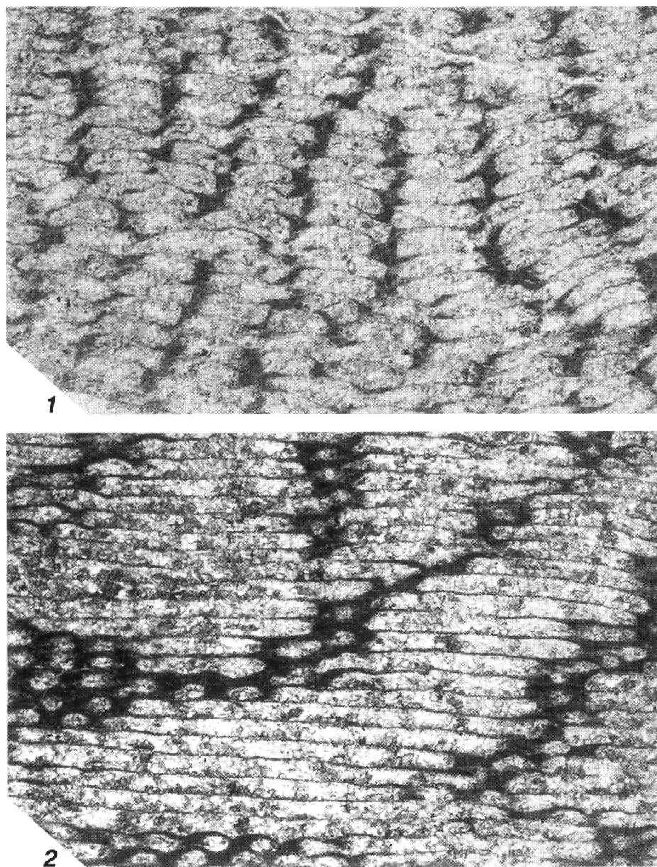
Fig. 5. Kitakamiia hamadai sp. nov., holotype, NSM PA14972, thin sections. 1, transverse sections of corallites, note intracolony columns, \times 14 . 2, longitudinal sections of corallites, \times 14 .
