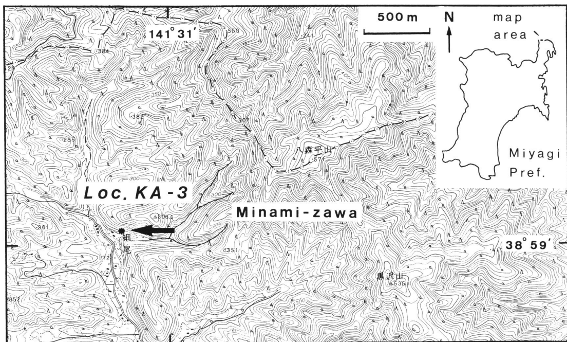
Fig. 1. Index map of the present coral locality in the Kamiyasse area, Kesennuma City, Miyagi Prefecture using 1: 25,000 map of "Shishiori" published by the Geographical Survey Institution.
