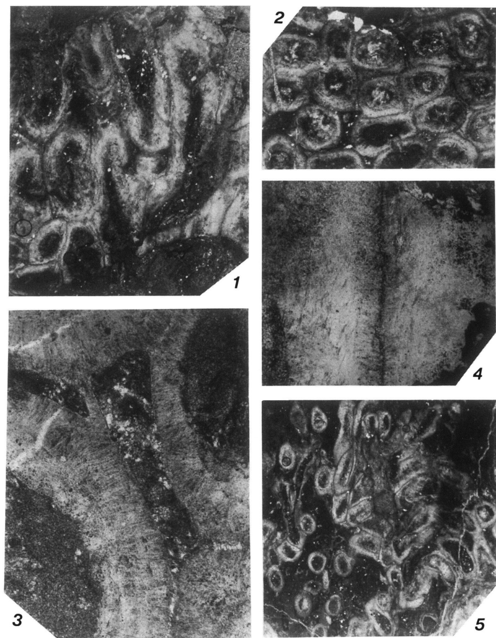
Fig. 3. Mandulapora jimboi sp. nov., thin sections. 1–4, holotype, NSM PA14959. 1, longitudinal to oblique sections of corallites in phacelo-cerioid portion, showing connecting tubule, \times 10 . 2, transverse sections of corallites in phacelo-cerioid portion, showing connecting tubule, \times 10 . 3, partial enlargement to show corallite wall structure and epithecal scale, transverse sections, \times 75 . 4, partial enlargement to show intercorallite wall structure, longitudinal section, \times 75 . 5, paratype, NSM PA 14960, oblique section of corallum, \times 5 .
