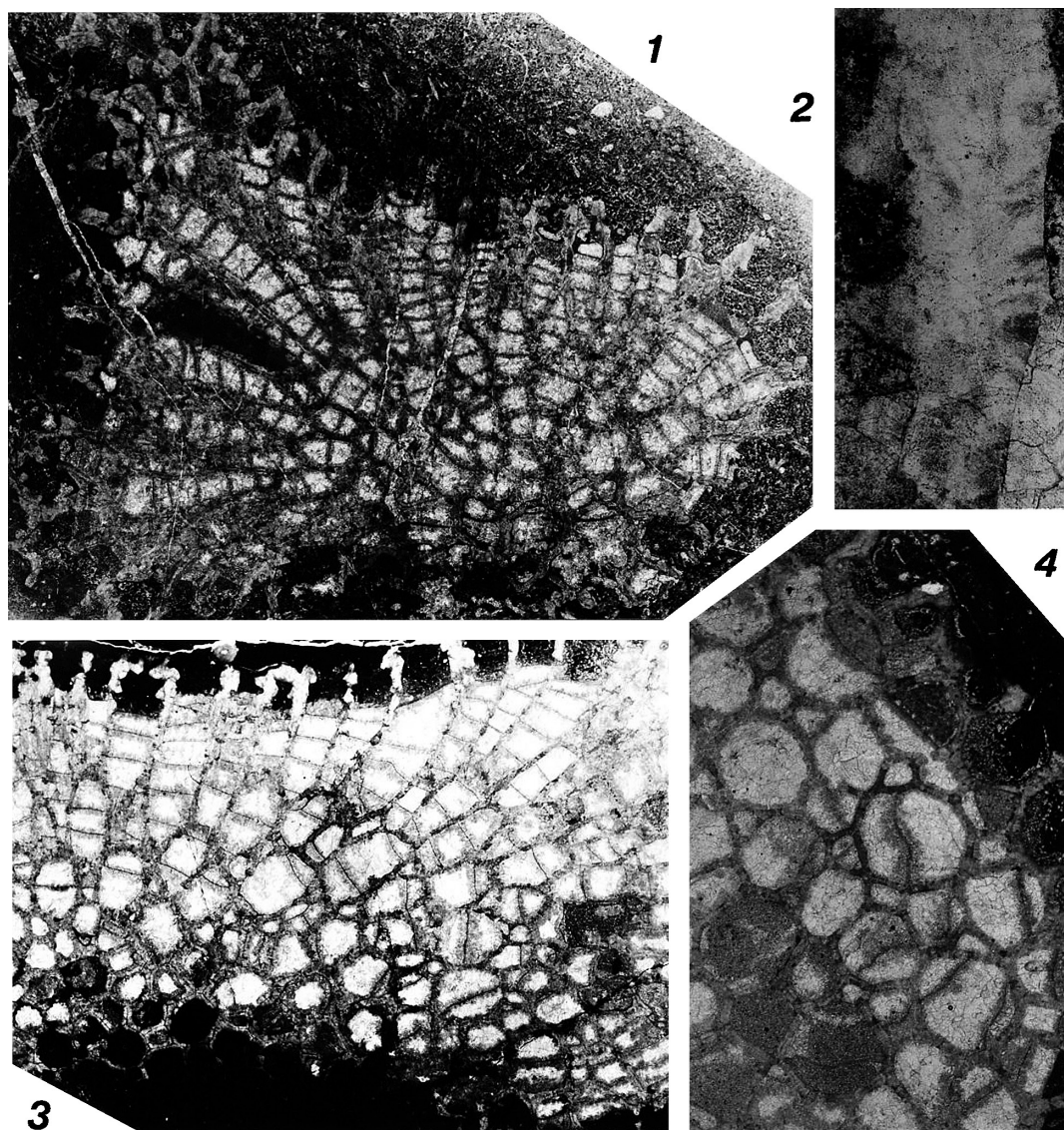
Fig. 2. Pachyfavosites hidensisformis (Mironova, 1961), thin sections. 1, NMNS PA17238, longitudinal section of corallum, \times 5 . 2, 3, NMNS PA17235. 2, partial enlargement to show intercorallite wall structure and septal spines, longitudinal section, \times 50 . 3, oblique section of corallum, \times 5 . 4, NMNS PA17237, transverse sections of corallites, \times 10 .
