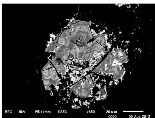
Fig. 7. Back-scattered image of pyrochlore. High- \text{Na}_2\text{O} and \text{CaO} but low- \text{H}_2\text{O} fields (light) and low- \text{Na}_2\text{O} and \text{CaO} but high- \text{H}_2\text{O} fields (dark) are observed. Minute flakes around crystal rim and along cracks of crystal (bright) are sklodowskite.
