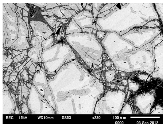
Fig. 8. Back-scattered image of microlite. Along cracks low- \text{Na}_2\text{O} and \text{CaO} but high- \text{H}_2\text{O} fields (slightly dark) are observed.
