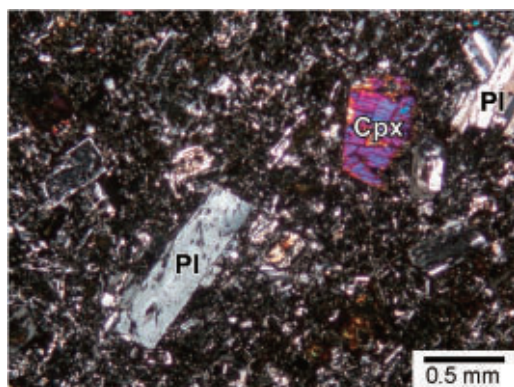
Fig. 6. Photomicrograph showing the texture of andesite discussed in this study. Pl means plagioclase and Cpx means clinopyroxene.
