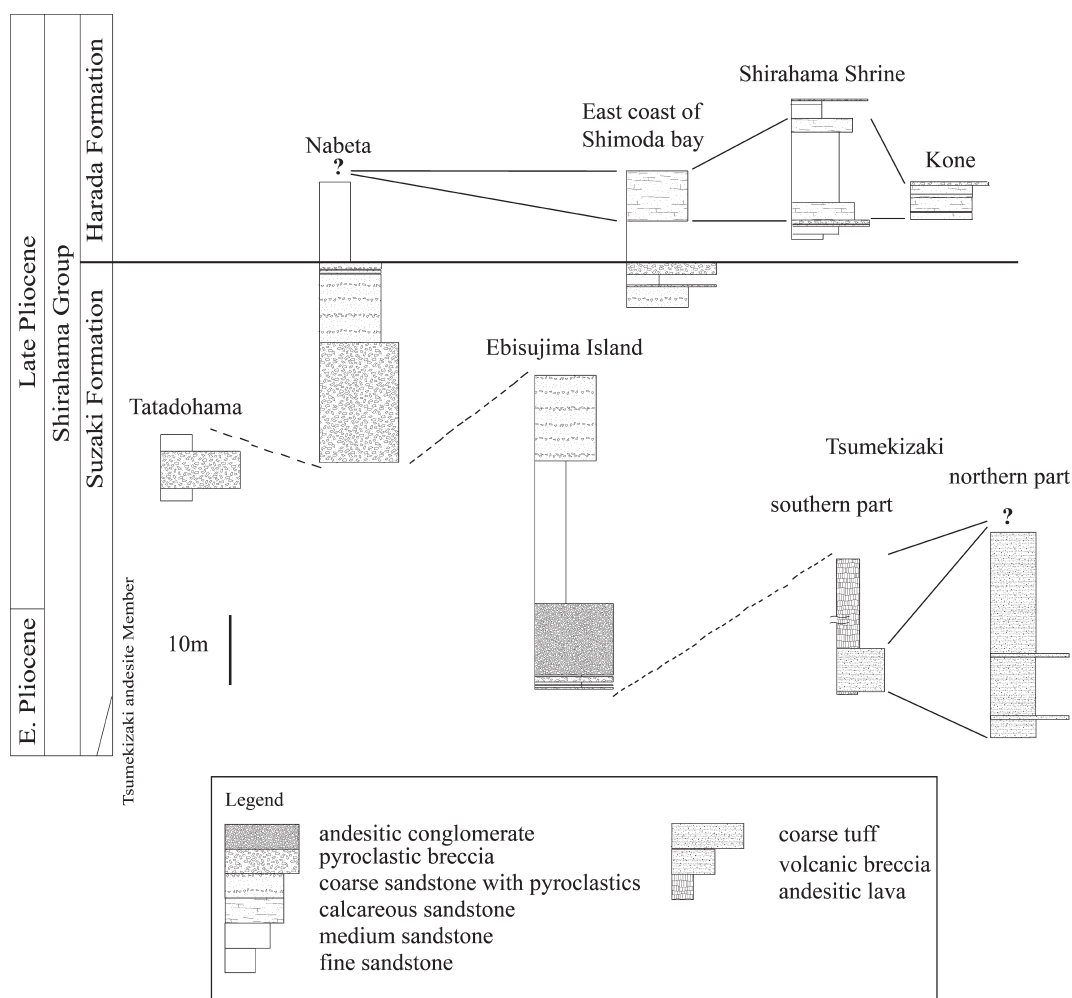
Fig. 3. Columnar sections within the study area except intrusive rocks.
