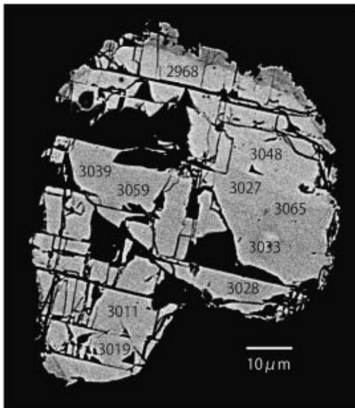
Fig. 8. The oldest monazite grain found from Sibuyan. Numbers in the grain are age shown as Ma. Obtained age is 3036 \pm 17 Ma.
