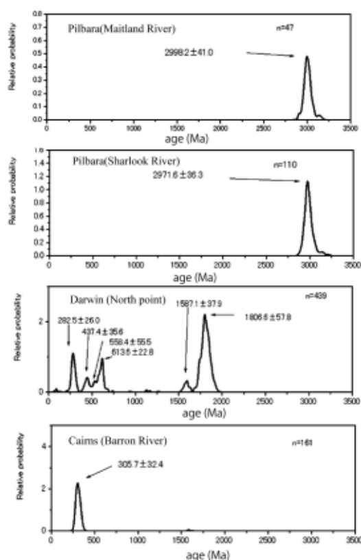
Fig. 7. Probability distribution diagrams of monazite ages in the sand samples collected from the northern part of the Australian Continent. Localities are shown in Fig. 1.
