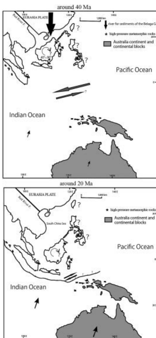
Fig. 10. Reconstruction models of Southeast Asia at around 40 and 20 Ma. Anticlockwise rotation by Schmidtke et al. (1990) and Fuller et al. (1999) has not been considered in the figures. A certain degree of rotation of Borneo will connect the Cretaceous granitic blocks in the continent and Borneo. Positions of plate subductions, Philippine and Taiwan islands have not been considered in the models.
