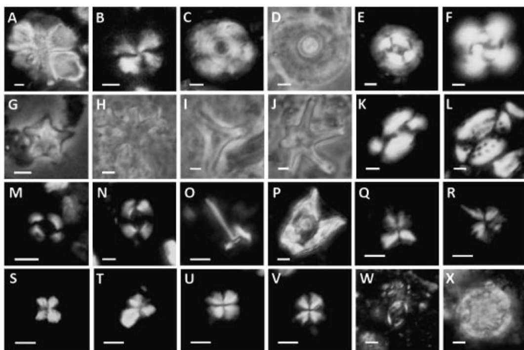
Fig. 4. Selected photomicrographs of calcareous nannofossils observed in the Pugo River section, La Union. XPL = cross-polarized image. PC = phase contrast image (scale bar = 2 microns). A. Ascidian spicule, XPL. B. Calcidiscus leptoporus , XPL. C–D. Calcidiscus macintyreii , XPL (C) and PC (D). E. Coccolithus pelagicus , XPL. F. Cyclicargolithus floridanus , XPL. G. Discoaster berggrenii , PC. H. Discoaster variabilis , PC. I. Discoaster triradiatus , PC. J. Discoaster sp., PC. K. Helicosphaera carteri , XPL. L. Pontosphaera sp., XPL. M. Reticulofenestra minuta , XPL. N. Reticulofenestra pseudumbilicus , XPL. O. Rhabdosphaera procera , XPL. P. Scyphosphaera pulcherrima , XPL. Q–R. Sphenolithus abies , 0° (Q) and 45° (R), XPL. S–T. Sphenolithus conicus , 0° (S) and 45° (T), XPL. U–V. Sphenolithus moriformis , 0° (U) and 45° (V), XPL. W. Syracosphaera sp., XPL. X. Thoracosphaera sp., XPL.
