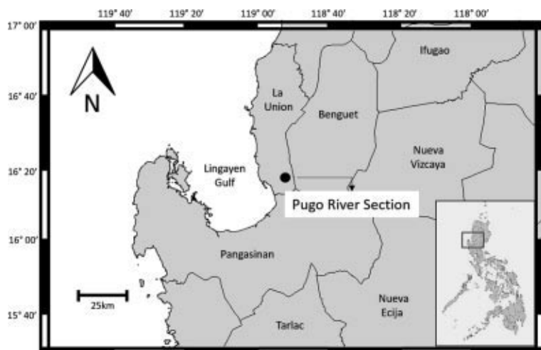
Fig. 1. Map of northern Luzon showing the location of the Pugo River Section in La Union Province, Philippines.
