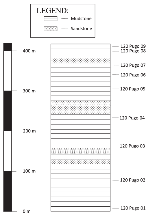
Fig. 3. Generalized stratigraphic column for the Pugo River Section in La Union Province. Relative stratigraphic positions of the samples are indicated in the column. The lithology of the outcrop is dominated by calcareous mudstones.
