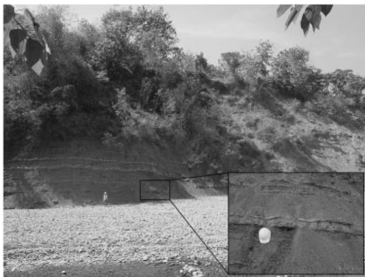
Fig. 2. Pugo River section in La Union Province. The outcrop is approximately 1 km in extent and 20m in height. The dominant lithologies are mudstones and siltstones, with minor calcareous sandstone and marly layers. Image on the lower right shows a close-up view of the boxed portion of the outcrop.
