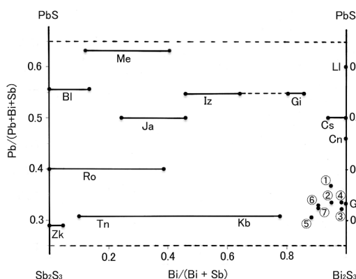
Fig. 4. PbS vs. \text{Sb}_2\text{S}_3 – \text{Bi}_2\text{S}_3 diagram. Fe, Cu and Ag are converted to Pb or Bi according to \text{Fe} = 2\text{Cu} , \text{Cu} + \text{Pb} = \text{Bi} , \text{Bi} + \text{Ag} = 2\text{Pb} (Moëlo et al. , 1995). Me, meneghinite; BL, boulangierite; Ro, robinsonite; Zk, zinkenite; Iz, izoklakeite; Gi, giessenite; Ja, Jaskólskiite; Tn, tintinaite; Kb, kobellite; Li, lillianite; Cs, cosalite; Cn, cannizzarite; Gb, galenobismutite. ①, Bärenbad (Paar et al. , 1983); ②, Bärenbad (Topa and Makovicky, 2012); ③, Felbertal 1 (Topa and Makovicky, 2012); ④, Felbertal 2 (Topa and Makovicky, 2012); ⑤, Hviezda (Pršek et al. , 2008); ⑥, Jishakuyama No. 4 (this study); ⑦, Jishakuyama No. 14 (this study).
