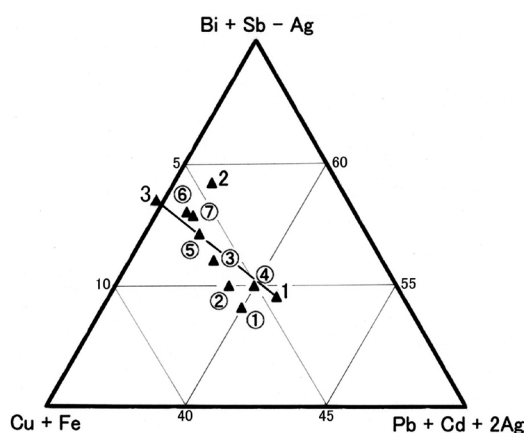
Fig. 5. (\text{Bi} + \text{Sb} - \text{Ag}) - (\text{Pb} + \text{Cd} + 2\text{Ag}) - (\text{Cu} + \text{Fe}) diagram (retouch in Fig. 2 reported by Topa and Makovicky, 2012). 1, \text{Fe}^{2+}\text{Pb}_9\text{Bi}_{12}\text{S}_{28} ; 2, \text{Cu}^+\text{Pb}_8\text{Bi}_{13}\text{S}_{28} ; 3, \text{Cu}^{+1.5}\text{Pb}_{7.75}\text{Bi}_{13}\text{S}_{28} . Circled numbers are same references as Fig. 4.
