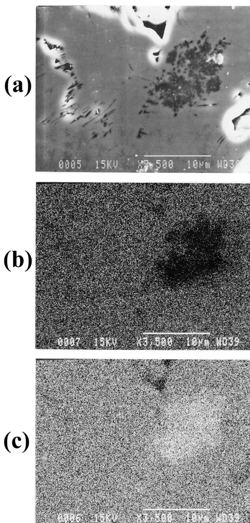
Fig. 16. (a) SEM image. (b) XES image of \text{CaK}\alpha . (c) XES image of \text{SiK}\alpha . Diopside in glimmerite. Ca leaches out from diopside and silicic components relatively concentrate there. Sample from the CVRD, Tapira (MG).
