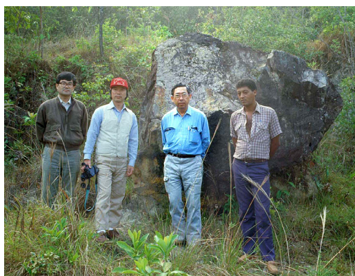
Fig. 19. The late Professor Kenkichi Fujimori in front of the block of Cadasite, Serrote, Poços de Caldas (SP). Photograph was taken on the 18th of October 1988 by Nobuhiko Haga. From left to right, Hiroyuki Horiuchi, Osamu Tachikawa, Professor Kenkichi Fujimori and Mr. Maruricio Antonio de Carvalho.
