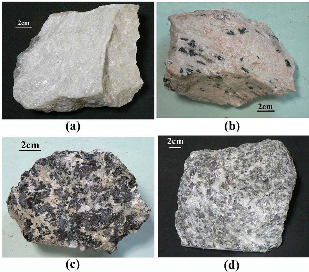
Fig. 3. Various carbonatites. Samples obtained at the Mines of Serrana S.A. de Mineração at Jacupiranga (SP). All of them contain calcite, dolomite and apatite as main constituents of rocks. Remarks are, (a) apatite is dominant, (b) some of magnetite, ilmenite are observed, (c) magnetite is dominant, and (d) olivine is included.
