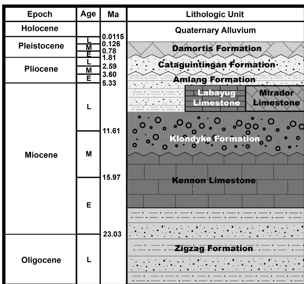
Fig. 2. Generalized stratigraphic column of the Ilocos-Central Luzon Basin at the vicinity of Sison, Pangasinan. The mudstone-limestone interbeds of NCC were previously assigned to the Amlang Formation based on lithological characteristics and depositional setting (Fernandez, 1996). Figure modified from Peña (2008).
