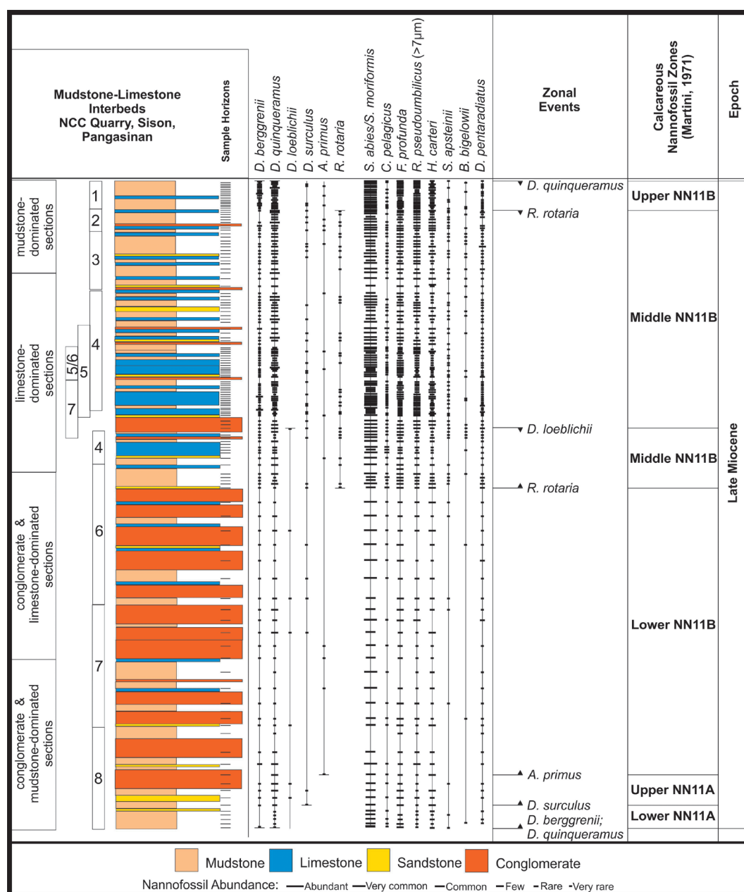
Fig. 4. Calcareous nannofossil biostratigraphic zonation and distribution of calcareous nannofossil zonal markers and other selected taxa in the mudstone-limestone interbeds of NCC Quarry area, Sison, Pangasinan. Thin horizontal bars at right side of the lithologic column indicate relative stratigraphic positions of the samples analyzed in this study (see also Appendix).
