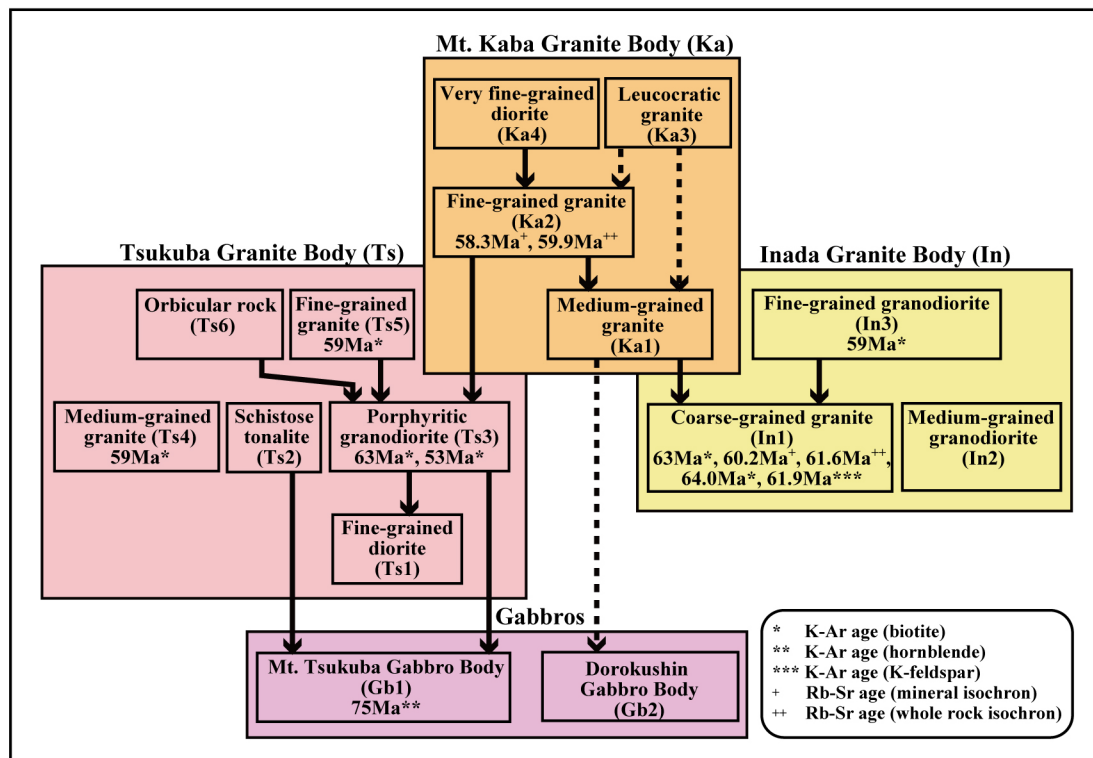
Fig. 3. Intrusive relationships of the Tsukuba plutonic bodies and radiometric ages (after Miyazaki et al. , 1996). Solid arrows show the relationships between two units confirmed at the outcrops. Dotted arrows show intrusive relationships estimated from the areal distributions of the rocks. Radiometric ages were from Kawano and Ueda (1966), Shiba et al. (1979), Arakawa and Takahashi (1988), Shibata and Uchiumi (1992) and Miyazaki et al. (1996)).
