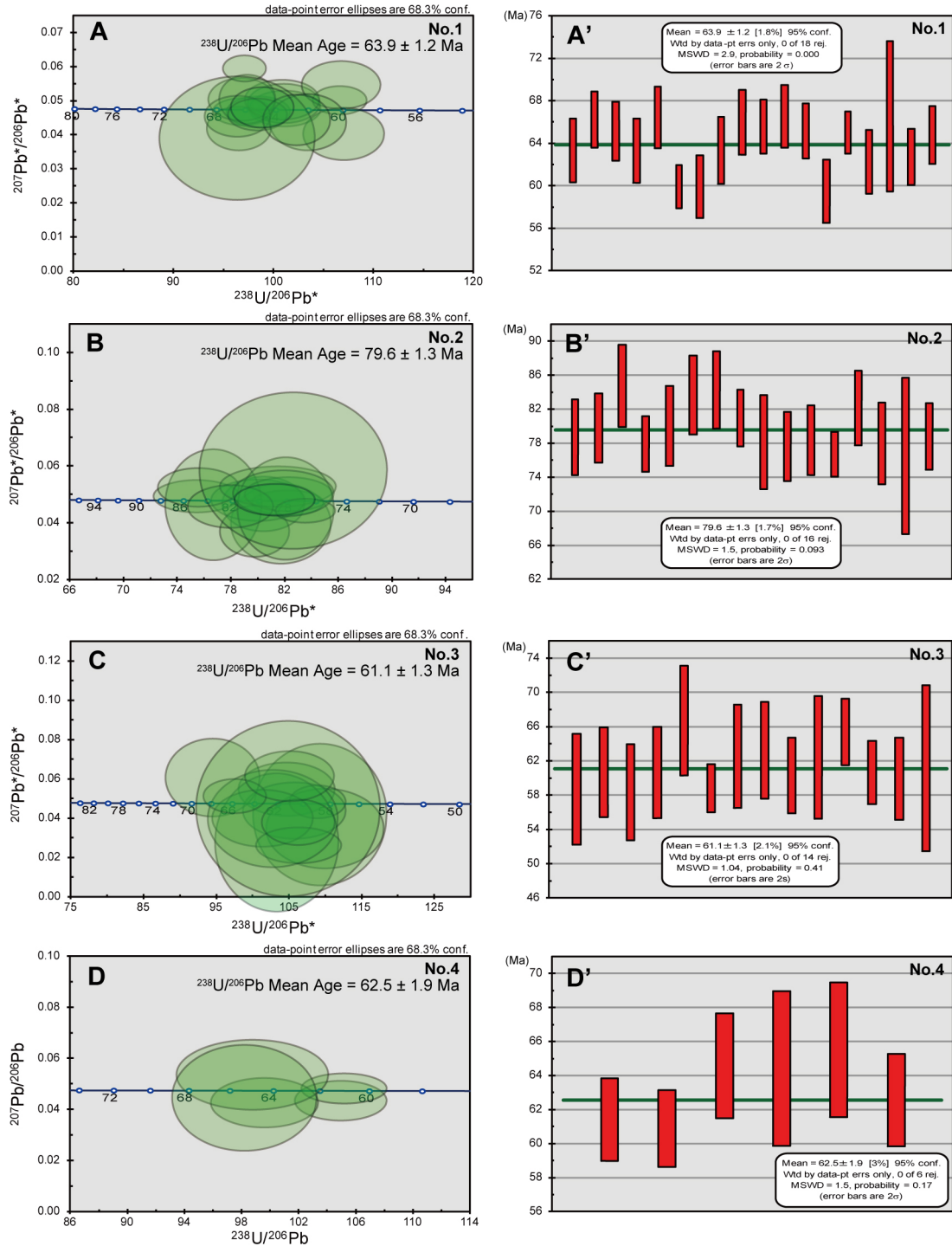
Fig. 5. Tera-Wasserburg concordia diagrams and age distribution plots of the analyzed granite samples. Left: Tera-Wasserburg concordia diagrams, right: age distribution plots. A & A': granite from the Mt. Kaba Body, sample 1. B & B': granite from the Tsukuba Body, sample 2. C & C': granite from the Tsukuba Body, sample 3. D & D': granite from the Tsukuba Body, sample 4. Error ellipses represent 68.3% confidence intervals. Quoted ages are weighted means of ^{207}\text{Pb} -corrected ^{206}\text{Pb}/^{238}\text{U} spot ages (n analyses, errors at 95% confidence intervals). Solid ellipses, analyses used in weighted mean age calculation; dotted ellipses, excluded analyses.
