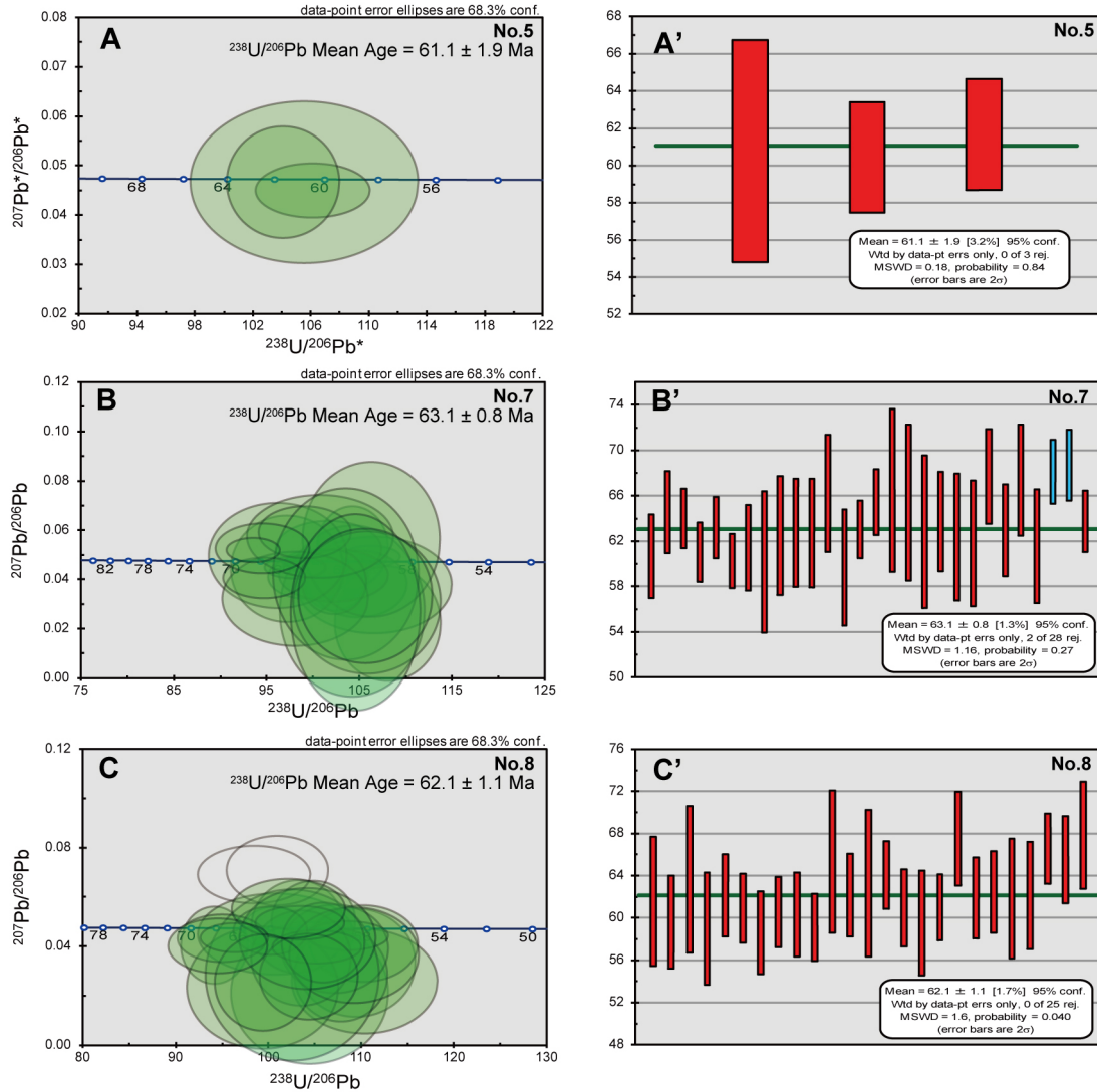
Fig. 6. Tera-Wasserburg concordia diagrams and age distribution plots of the analyzed gabbro samples. Left: Tera-Wasserburg concordia diagrams, right: age distribution plots. A & A': anorthositic pyroxene gabbro from the Mt. Tsukuba Body, sample 5. B & B': pyroxene gabbro from the Mt. Tsukuba Body, sample 7. C & C': hornblende gabbro from the Dorokushin Body, sample 8. Error ellipses represent 68.3% confidence intervals. Quoted ages are weighted means of ^{207}\text{Pb} -corrected ^{206}\text{Pb}/^{238}\text{U} spot ages (n analyses, errors at 95% confidence intervals). Solid ellipses, analyses used in weighted mean age calculation; dotted ellipses, excluded analyses.
