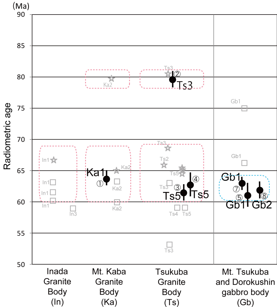
Fig. 7. The radiometric ages of the Tsukuba plutonic rocks. White squares are from Kawano and Ueda (1966), Shiba et al. , (1979), Arakawa and Takahashi (1988), Miyazaki et al. (1966), Shibata and Uchiumi (1992). White stars are from Yokoyama et al. (2016). Black circles are from this study.
