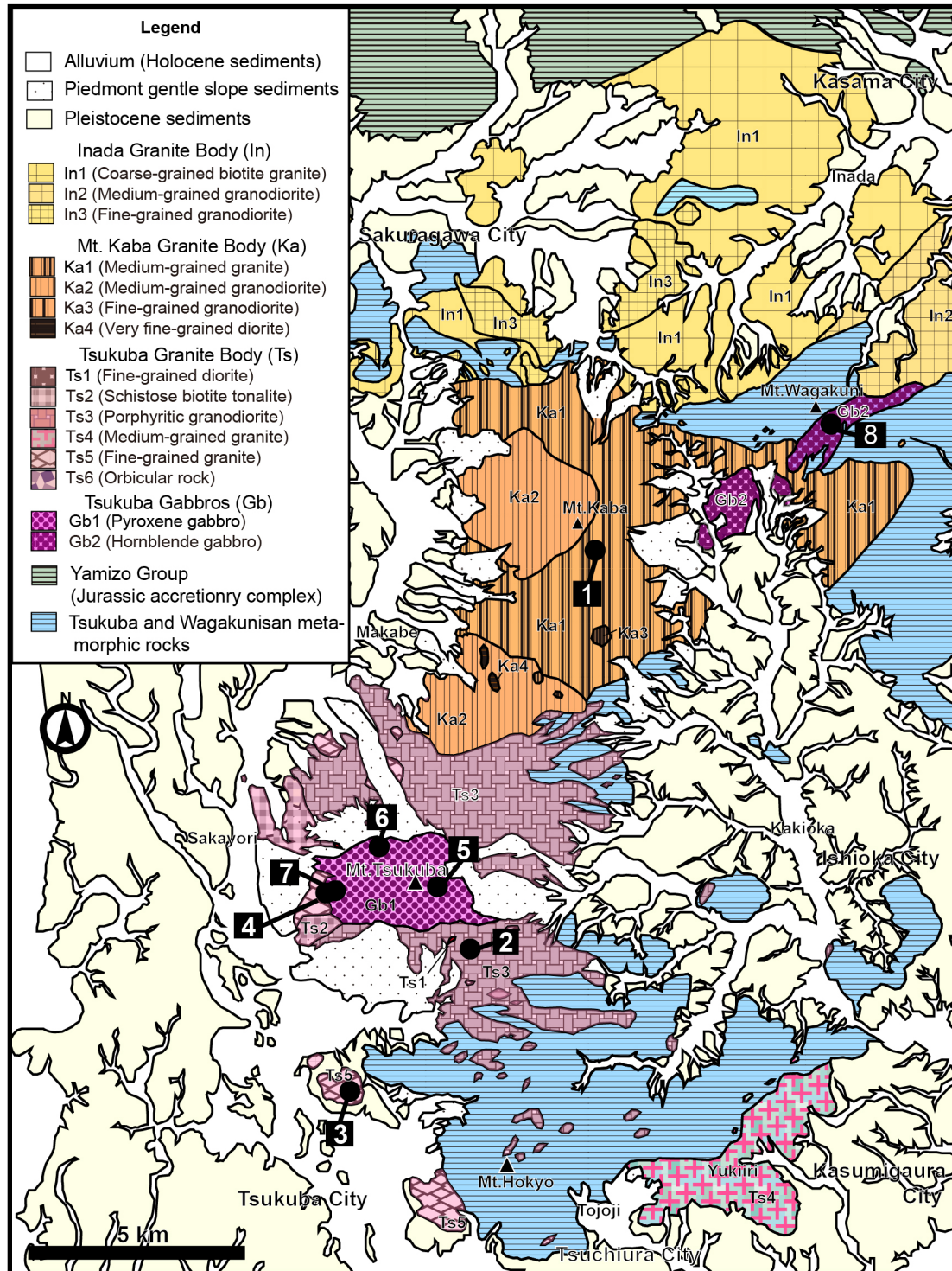
Fig. 1. Geological map of the Tsukuba area (partly revised after Takahashi, 2006). Numbers in black squares are analyzed samples.
