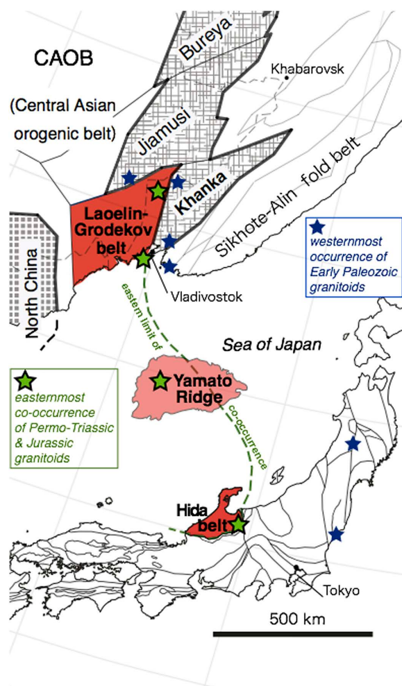
Fig. 4. Geotectonic map of the circum-Sea of Japan, East Asia (compiled from Khanchuk et al. , 1996; Wilde, 2015; Isozaki et al. , 2010), showing relative positions of the LG belt in Primorye, the Yamato ridge in the middle of the Sea of Japan, and the Hida belt in central Japan. Green stars represent the easternmost (Pacific-side) localities of co-occurred Permo-Triassic and Jurassic granitoids in the LG belt, Yamato Ridge, and Hida belt (Ma et al. , 2014; Lelikov et al. , 1996), and blue ones the westernmost locality of Early Paleozoic granitoids on the Pacific side (Sakashima et al. , 2003; Tagiri et al. , 2011; Kruk et al. , 2012; Isozaki et al. , 2015). The geologic similarities, particularly in the two-fold granitoid ages of the Permo-Triassic and Jurassic, suggest the primary consanguinity among the LG belt, Yamato Ridge, and Hida belt, although they have been separated from each other since the Miocene opening of the Sea of Japan. Note that the Hida belt can be correlated neither with North China block nor Khanka block but uniquely to the LG belt.
