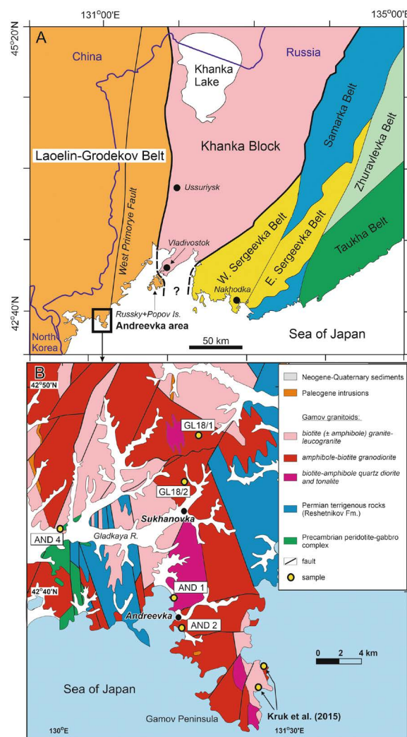
Fig. 1. Index map of Laelin-Gorodekov belt after Malinovsky and Golozubov (2021) (A), and geologic sketch map (B) of Andreevka area in Laelin-Gorodekov belt in southwestern Primorye, Far East Russia, after State Geological map of the Russian Federation on a Scale 1:200,000 Khanka Series. sheets K-52-XII and K-52-XVIII (2004) and Kruk et al. (2015) with five sample localities of granitoids for dating in this study.
