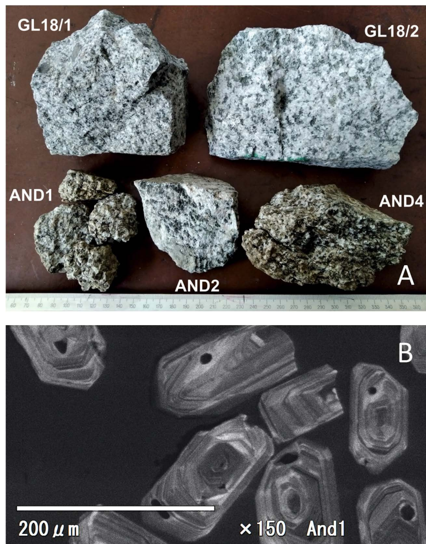
Fig. 2. Photographs of five hand specimens of Gamov granitoids (A) and examples of cathodoluminescence images of dated zircons from AND1 with oscillatory zoning texture (B).
