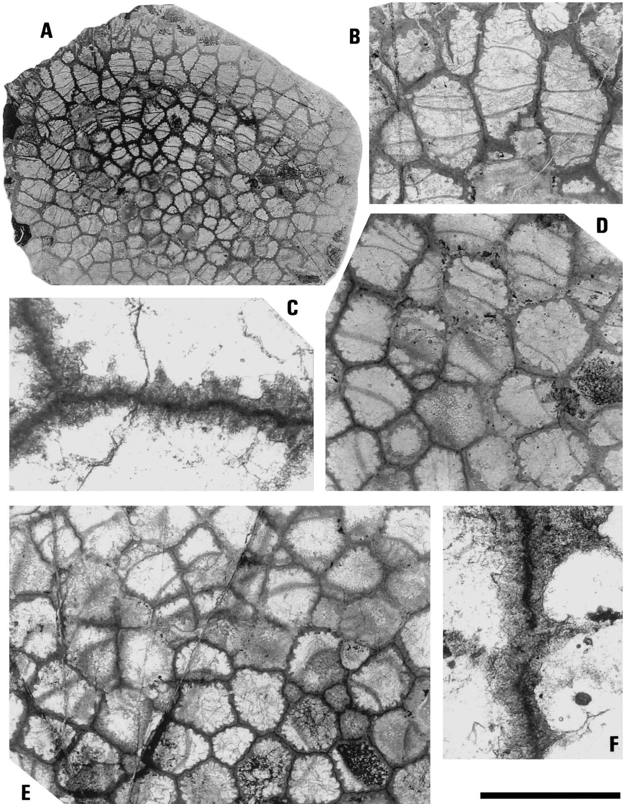
Fig. 4. Protomichelinia favositoides (Girty, 1907), thin sections. A, B, D , J73. A , transverse section of corallum. B , partial enlargement to show oblique sections of corallites. D , partial enlargement to show transverse sections of corallites. C, E, F , J59. C , partial enlargement to show intercorallite wall structure, transverse section. E , partial enlargement to show transverse sections of corallites. F , partial enlargement to show intercorallite wall structure and details of septal spines, longitudinal section. Scale bar: A = 12 mm; B, D, E = 4 mm; C, F = 0.7 mm.
