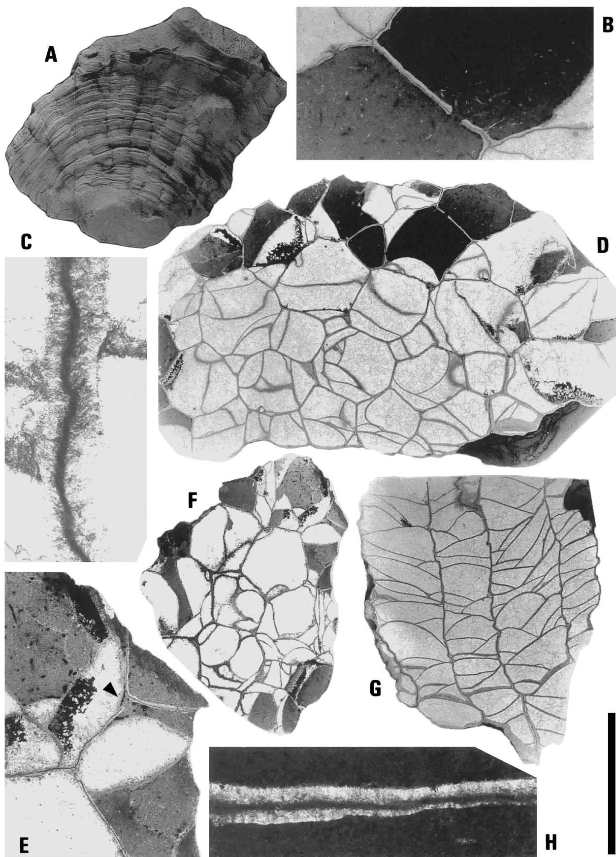
Fig. 3. Julfamichelinia allata (Tchudinova in Ruzhentsev and Sarycheva, 1965). A–D, G, H, NMNS PA20010. A, side view of corallum. B, partial enlargement to show details of mid-wall pore, transverse thin section. C, partial enlargement to show intercorallite wall structure, longitudinal thin section. D, transverse thin section of corallum. G, longitudinal thin section of corallum. H, partial enlargement to show intercorallite wall structure, transverse thin section. E, F, G86, thin section. E, partial enlargement to show details of angle pore (arrow), transverse section. F, transverse section of corallum. Scale bar: A = 24 mm; B, E = 4 mm; C, H = 0.7 mm; D, F, G = 12 mm.
