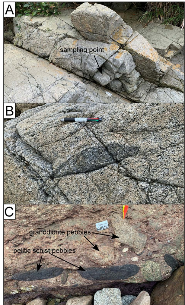
Fig. 3. Photographs of typical outcrops; A: An outcrop of the Oseto granodiorite (sample locality of OST). B: Lenticular MME in the Oseto granodiorite. C: Basal conglomerate of the Paleogene sedimentary sequence overlying the Oseto granodiorite. D and E: A view of Kotatejima Island and the sampling point of KTT, respectively. F and G: A view of Otateshima Island and the sampling point of OTT, respectively. H and I: A view of Irose Islet and the sampling point of IRS, respectively. J: The sampling point of ENS. K: the sampling point of HRK.
