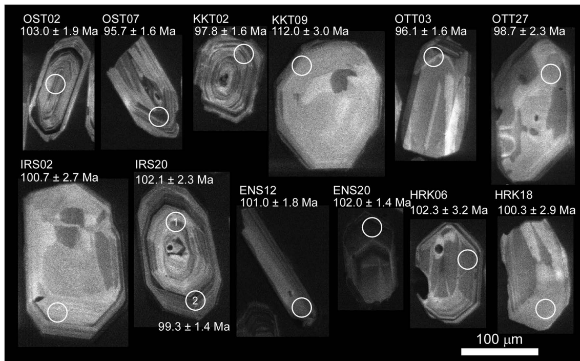
Fig. 4. Cathodoluminescence images of analyzed section of typical zircon grains from the samples. Circles in the images indicate points analyzed by LA-ICP-MS and are approximately 25 \mu\text{m} in diameter.
