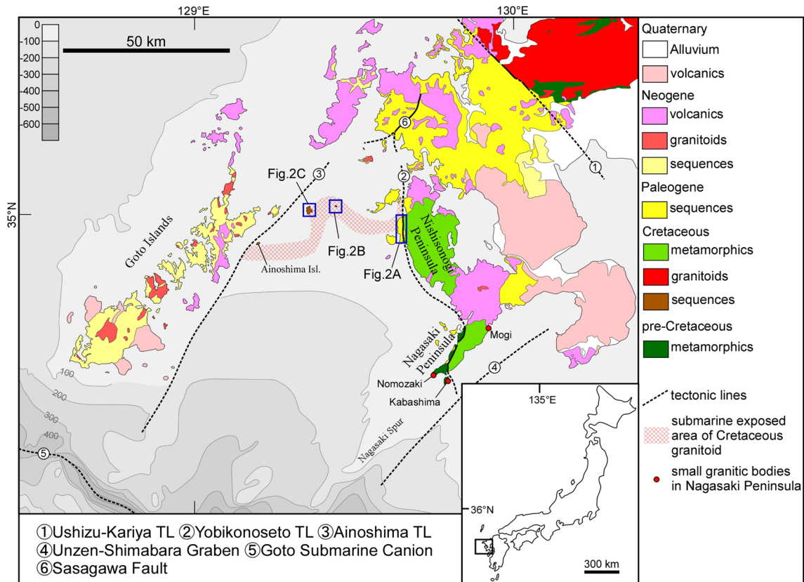
Fig. 1. Geological map of northwestern Kyushu. Submarine exposed area of Cretaceous granitoids is from Tachibana (1962).
