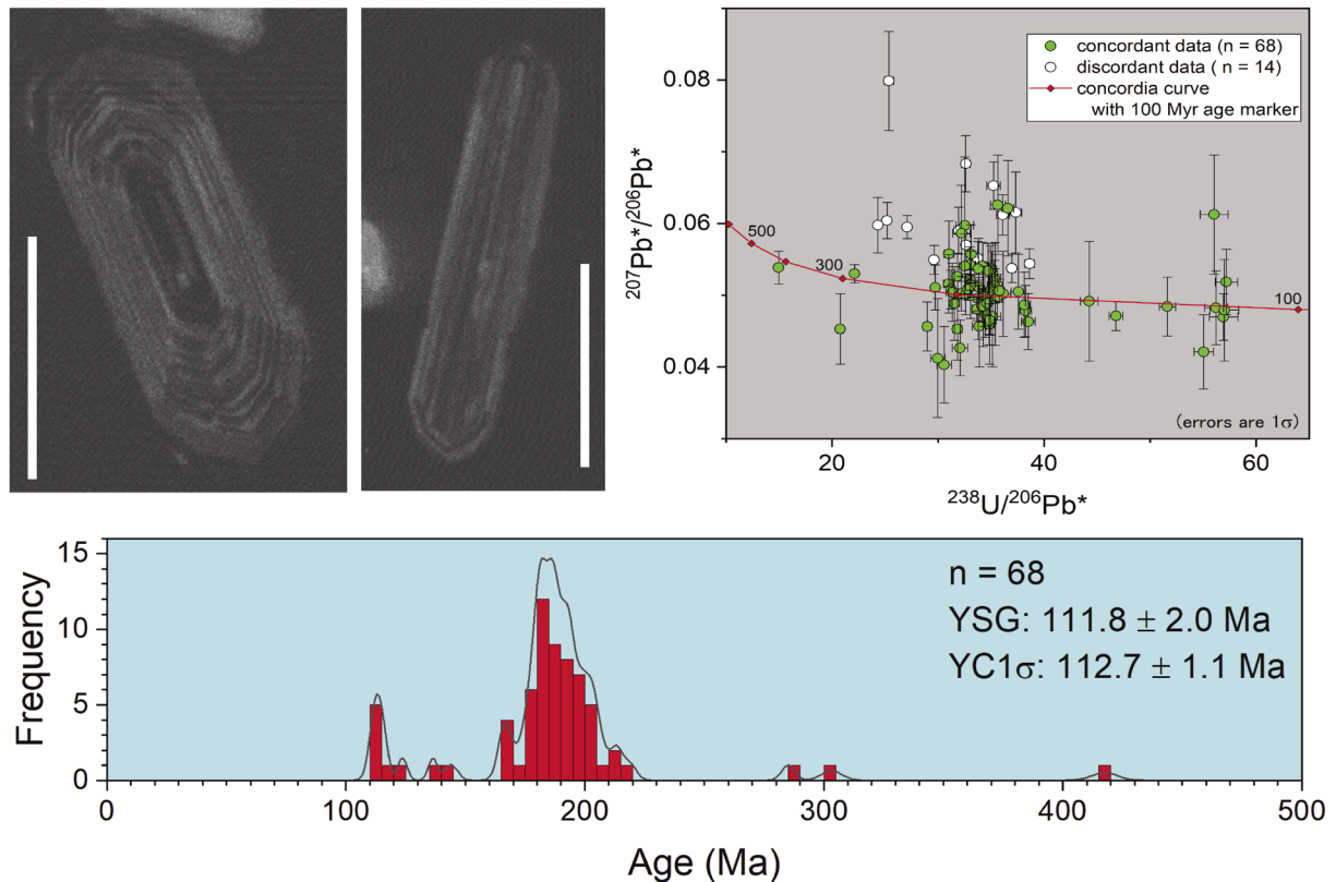
Fig. 4. Examples of cathode-luminescence image of dated zircons with scale bar of 100 micrometer (A), concordia diagram (B), and U-Pb age spectrum of detrital zircons in histogram and probability density curve (C) for analyzed sandstone (Sample PR6) from the Lipovtsy Fm, Nikan Group, in the Razdol'naya coal field, Primorye.
