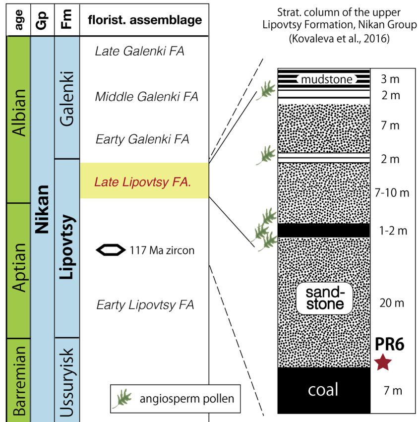
Fig. 2. Correlation diagram of the Nikan Group in southern Primorye (left: Kosenko et al. , 2021) and the stratigraphic column of the study section at the Porechye open-pit coal mine near the study section (right: Kovaleva et al. , 2016) with the sample horizon (red star). Note that the first appearance horizon of angiosperm (pollen) in the Upper Lipovtsy Fm is nearly 20m above the horizons of dated sample PR6.
