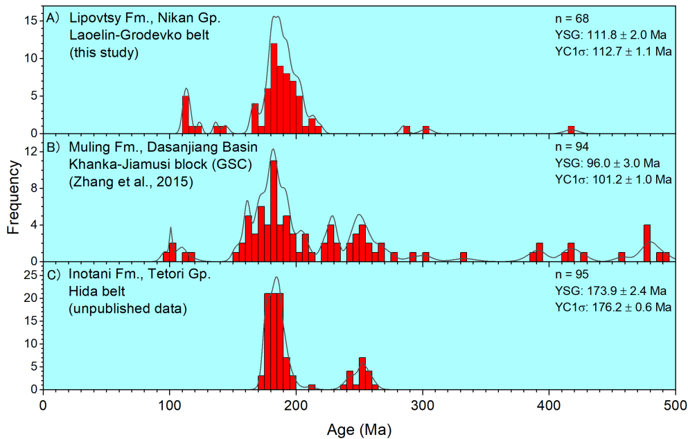
Fig. 6. Comparison of age spectra of detrital zircons among neighboring belts/units. A: Lipovtsy Fm (Nikan Gp) in L-G belt, Primorye (Sample PR6, this study), B: Muling Fm in Jiamusi block, NE China (Zhang et al. , 2015), C: Inotani Fm (Tetori Gp) in Hida belt, Japan (Isozaki et al. , in review).
