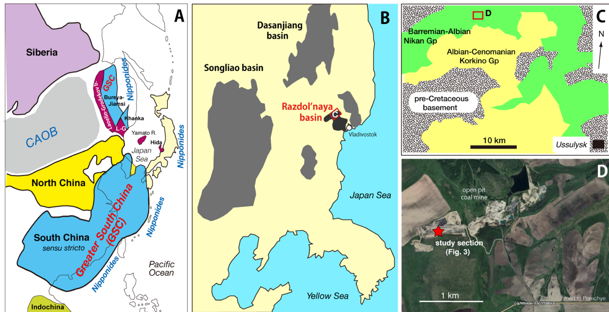
Fig. 1. Index geotectonic map of Far East Asia (A; modified from Isozaki, 2019), index map of major Cretaceous basins (gray) with the Razdol'naya coal basin (dark gray) in South Primorye, Russia (B; simplified from Kirillova, 2018), local geologic map of the northern Razdol'naya basin (C; simplified from Volynets and Bugdaeva, 2017) with the location of study section (red square), and a satellite image (Google Earth) of the study section in the open-pit coal mine near Porechye (D).
