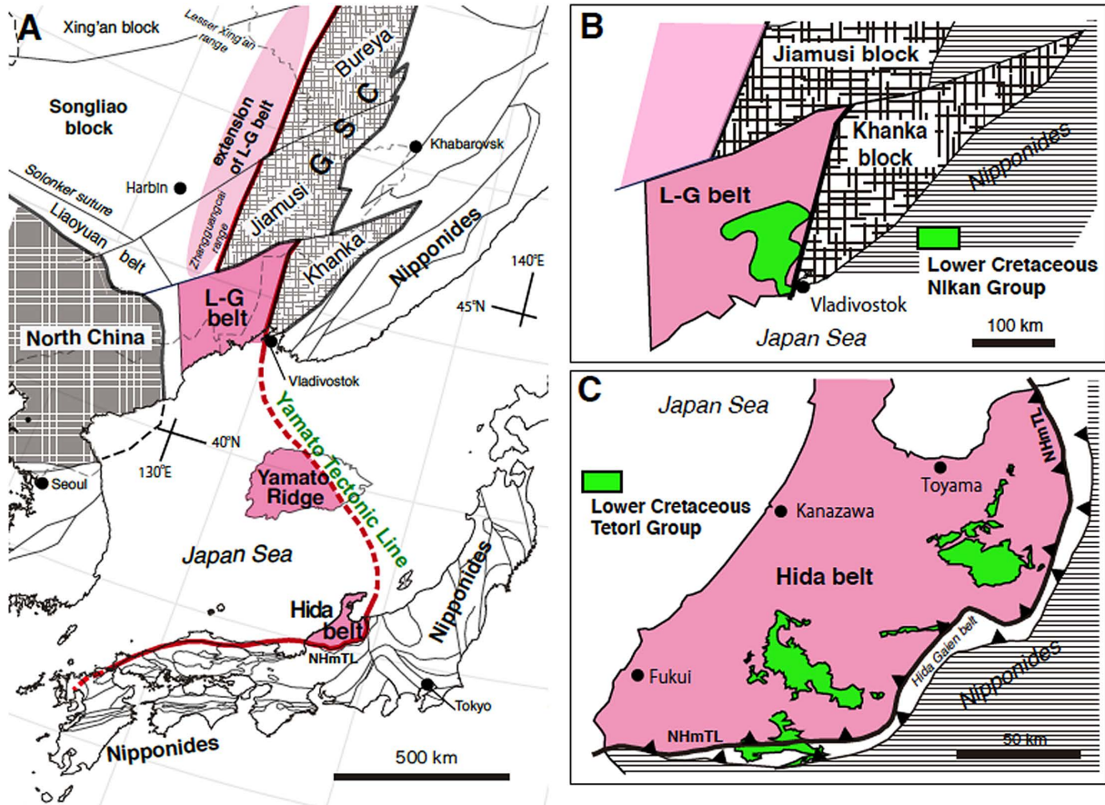
Fig. 7. Geotectonic framework of Far East Asia (A; modified from Isozaki et al. , 2023) and distribution of Lower Cretaceous non-marine strata in the Laoelin-Grodekov belt, Primorye (B: the Nikan Group; Krillova, 2018) and that in the Hida belt, central Japan (C: the Tetori Group; Matsukawa et al. , 2014).
