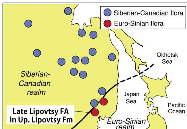
Fig. 5. Albian (late Early Cretaceous) paleofloristic biogeography in Far East Asia (simplified from Kirillova, 2018).
