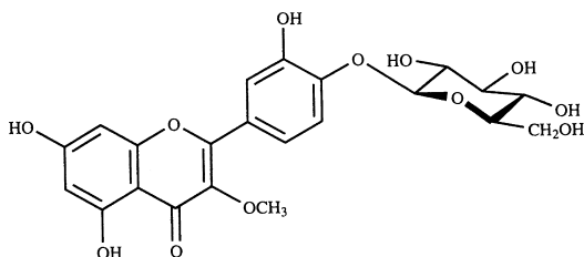
Fig. 8. Quercetin 3-methyl ether 4'- O -glucoside (Neochilenin, 9 ).
