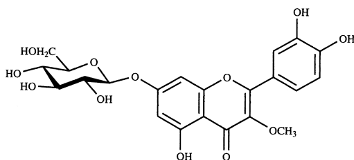
Fig. 7. Quercetin 3-methyl ether 7- O -glucoside (Transilin, 8 ).
