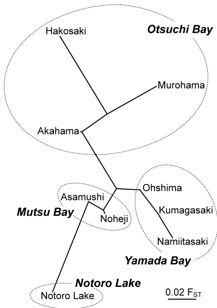
Fig. 2 Neighbor-joining (NJ) tree based on F_{ST} values (Weir and Cockerham, 1984) among Zostera caespitosa sites in this study.
