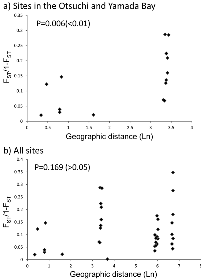
Fig. 3. Isolation-by-distance (IBD) used Mantel tests for Zostera caespitosa sites in this study based on F_{ST} as genetic distance. a) Six sites within the Otsuchi Bay and Yamada Bay; b) All Z. caespitosa sites. Pairwise genetic differentiation between populations were linearized and plotted against the geographic distance.
