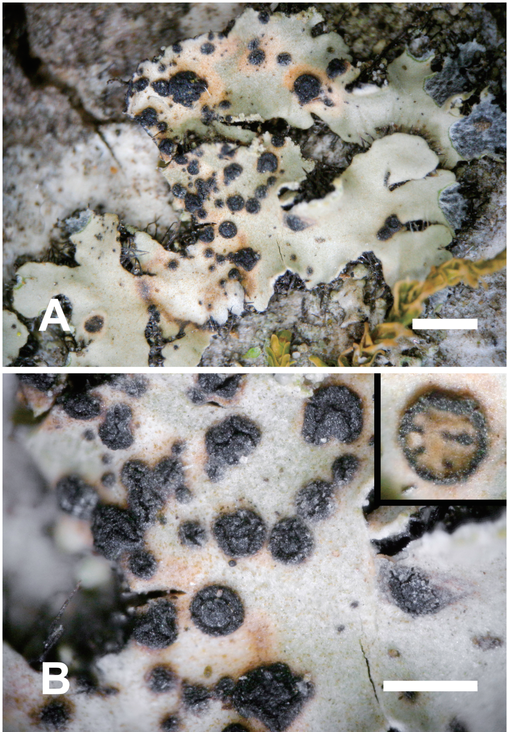
Fig. 1. Opegrapha phaeophysciae (Frisch 12/Jp183, TNS). A. Growth habit on Phaeophyscia limbata . B. Group of ascomata (the small picture shows a horizontal section through an ascoma with marginally divided hymenium). Scale bars: A = 1.0 mm, B = 0.5 mm.
