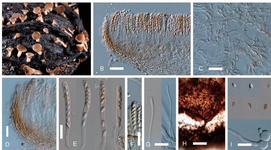
Fig. 4. Lambertella corni-marisi (TNS-F-40083). A. Fresh apothecia on fallen fruits of Torreya nucifera . B. Vertical section of an apothecium. C. Close up of medullary excipulum. D. Close up of ectal excipulum at the margin. E. Asci. F. Reaction of ascus apex to MLZ. G. Paraphyses. H. Surface structure in blackened area on host substrate. I. Hyaline ascospores, brown ascospores and germinating ascospores. Bars, B, 40 \mu\text{m} ; C–I, 20 \mu\text{m} .
