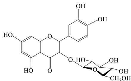
Fig. 5. Chemical structure of quercetin 3- O -glucoside ( O3 ) from Thermopsis barbata .
