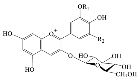
Fig. 3. Chemical structures of anthocyanins from Thermopsis barbata .
