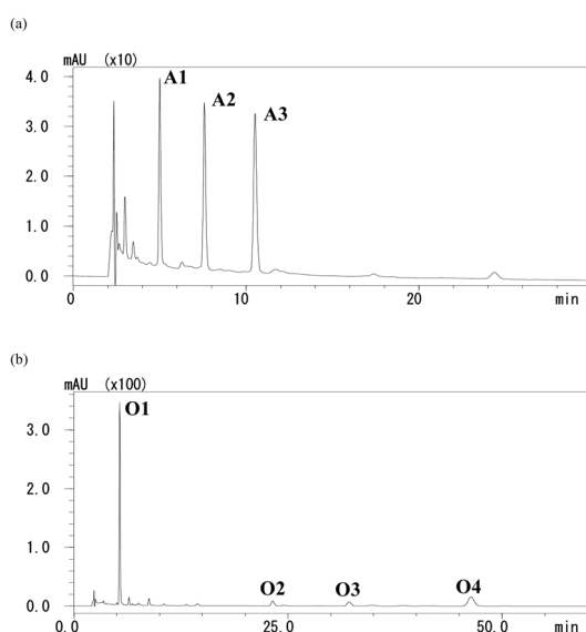
Fig. 2. HPLC chromatogram of MAW extracts from Thermopsis barbata .
