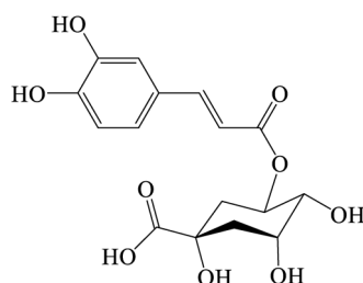
Fig. 4. Chemical structure of chlorogenic acid ( O1 ) from Thermopsis barbata .
