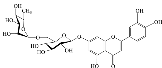
Fig. 6. Chemical structure of luteolin 7- O -rutinoside ( O4 ) from Thermopsis barbata .
