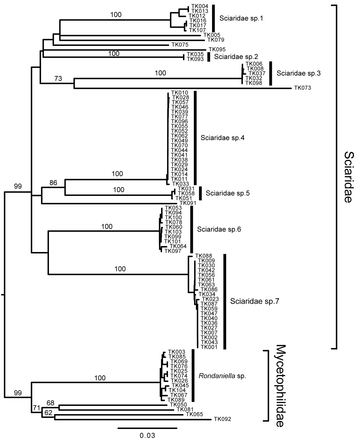
Fig. 2. A neighbor-joining tree of 87 fungus gnat (Sciaridae and Mycetophilidae) individuals collected in the present study based on 624-bp of mitochondrial cytochrome oxidase subunit I gene. Bootstrap supports for nodes above the species-level are shown (only when >50%).
