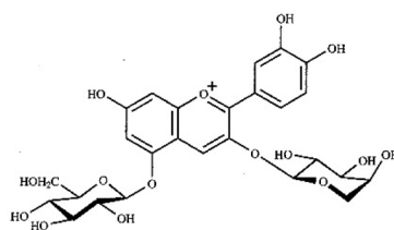
Fig. 1. Cyanidin 3- O -arabinoside-5- O -glucoside ( A1 ).
