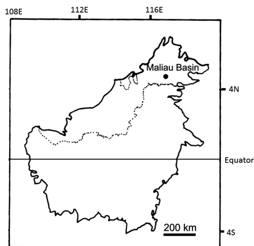
Fig. 1. Map of Borneo Island and collection sites. The mid line shows the equator. Dotted line shows the boundary of Indonesia and Brunei.
