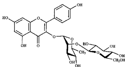
Fig. 1. Kaempferol 3- O -glucosyl-(1→2)-rhamnoside.
