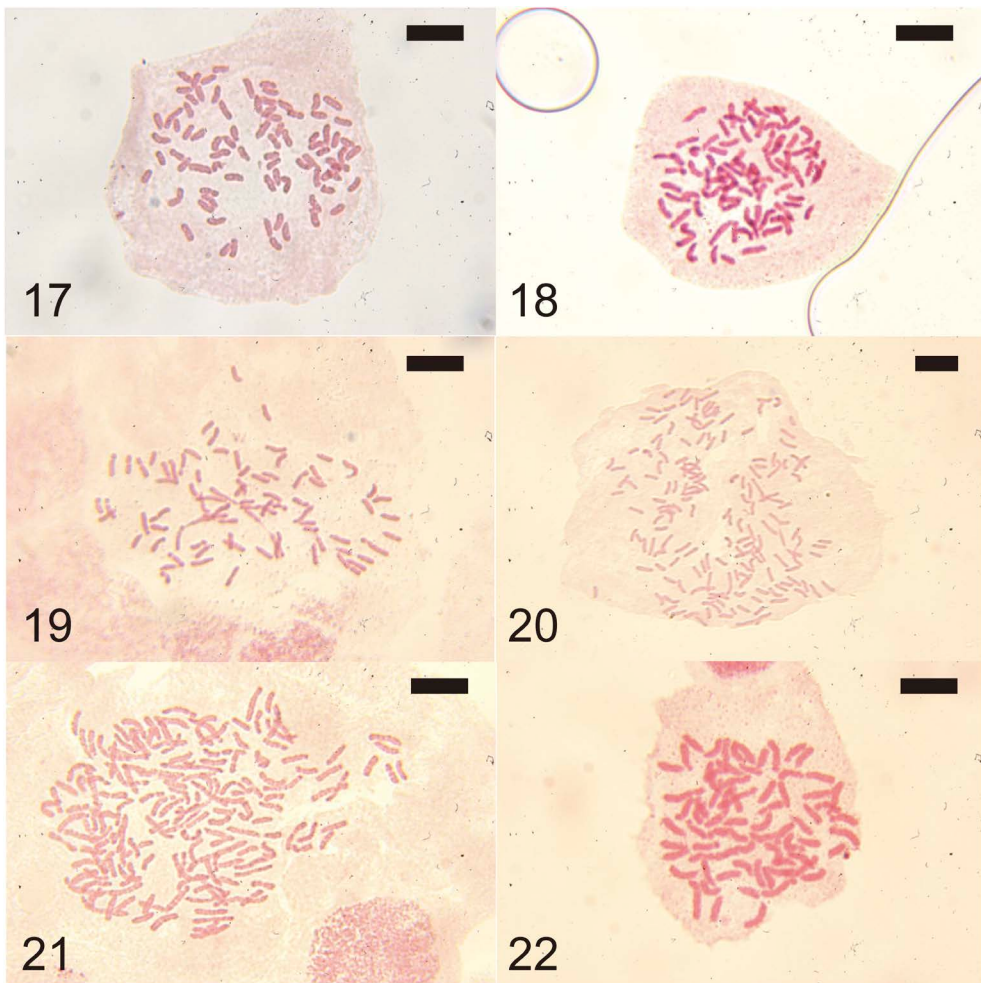
Figs. 17–22. Microphotographs of mitotic metaphase chromosomes. Scale bars = 10 \mu m. 17. Arachniodes cavaleriei ( 2n = 82 ). 18. Ctenitis microlepigera ( 2n = 82 ). 19. Dryopteris lunanensis ( 2n = 82 ). 20. Arthropteris palisotii ( 2n = 164 ). 21. Tectaria fauriei ( 2n = 160 ). 22. Microsorium rubidium ( 2n = 72 ).
