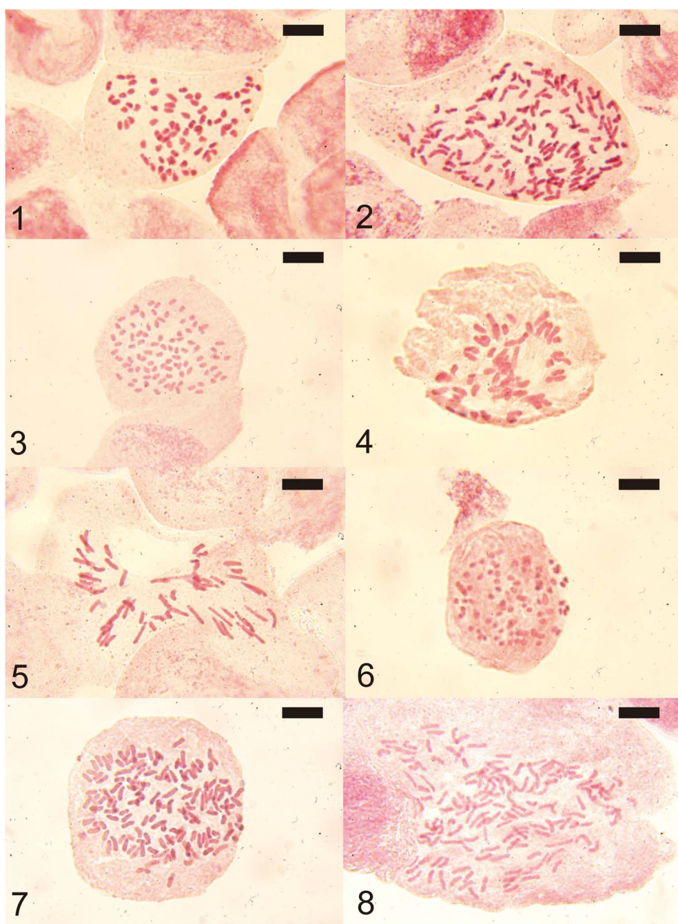
Figs. 1–8. Microphotographs of mitotic metaphase chromosomes. Scale bars = 10 \mu m. 1. Angiopteris fokiensis ( 2n = 80 ). 2. Ptisana boninensis ( 2n = 156 ). 3. Cheilanthes chusana ( 2n = 90 ). 4. Pteris kawabatae ( 2n = 58 ). 5. Pteris setulosocostulata ( 2n = 58 ). 6. Acystopteris tenuisecta ( 2n = 84 ). 7. Asplenium formosae ( 2n = 144 ). 8. Thelypteris erubescens ( 2n = 144 ).
