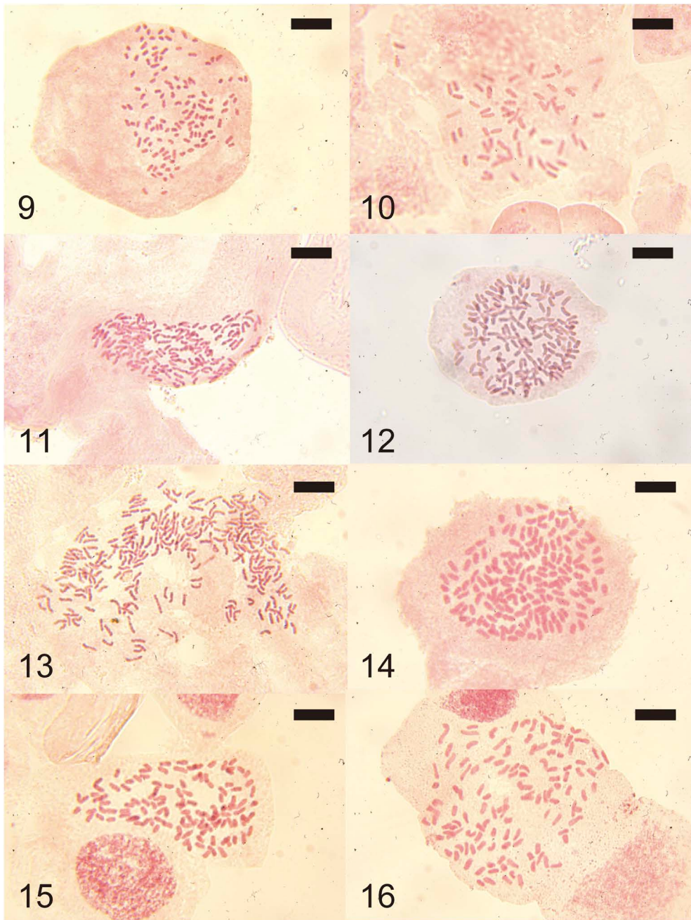
Figs. 9–16. Microphotographs of mitotic metaphase chromosomes. Scale bars = 10 \mu m. 9. Thelypteris gracilescens ( 2n=132 ). 10. Blechnum hancockii ( 2n=62 ). 11. Athyrium palustre ( 2n=160 , Nagasaki Pref.). 12. Athyrium silvicola ( 2n=160 ). 13. Athyrium spinescens ( 2n=240 ). 14. Deparia longipes ( 2n=160 , Gifu Pref.). 15. D. longipes ( 2n=120 , Wakayama Pref.). 16. Diplazium megaphyllum ( 2n=123 ).
