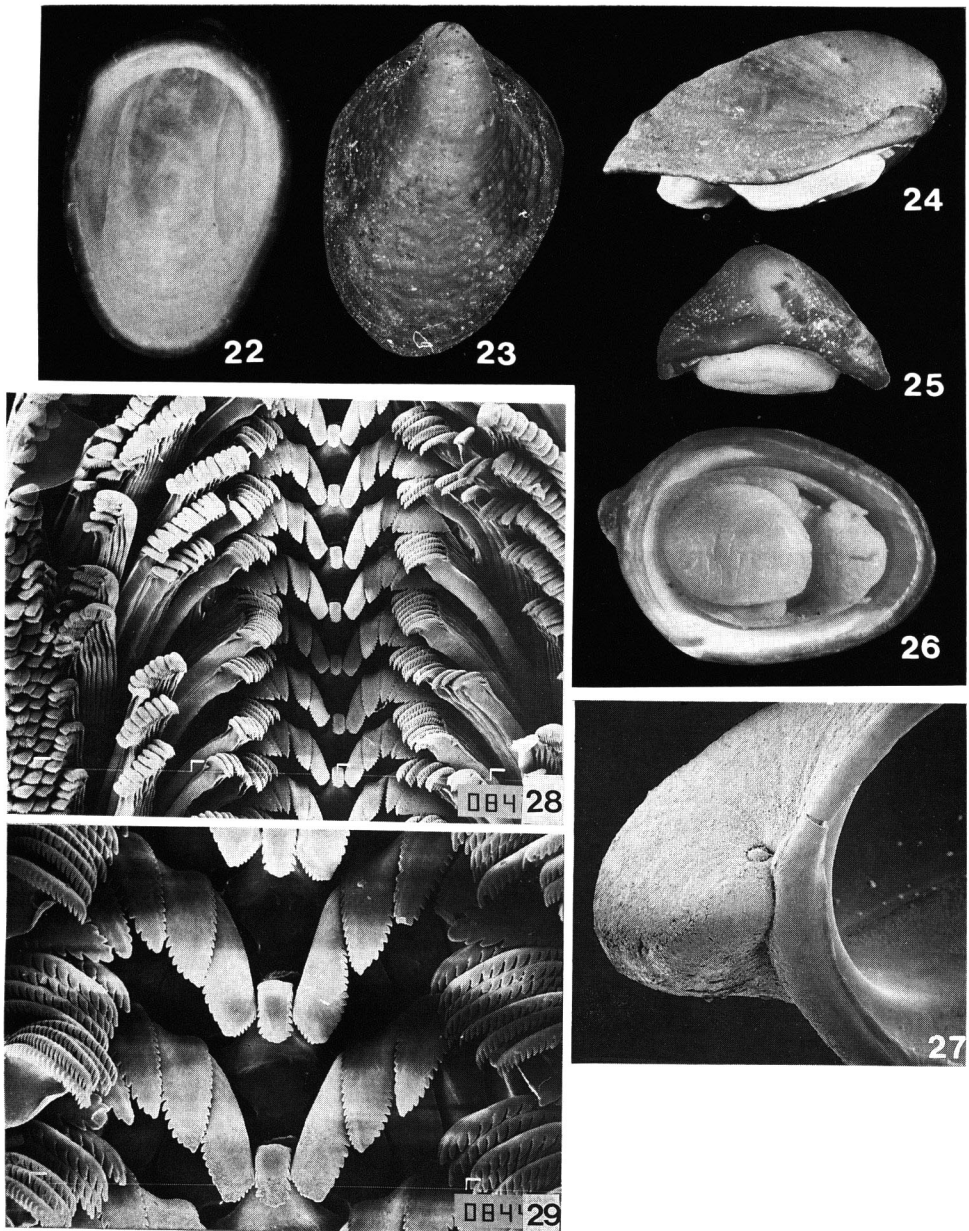
Figs. 22–29. Peltospiridae
