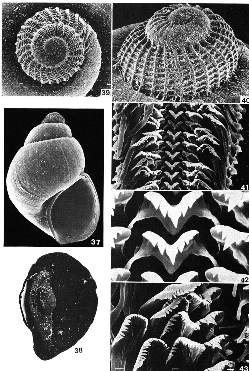
Figs. 37-43. Elachisinidae
