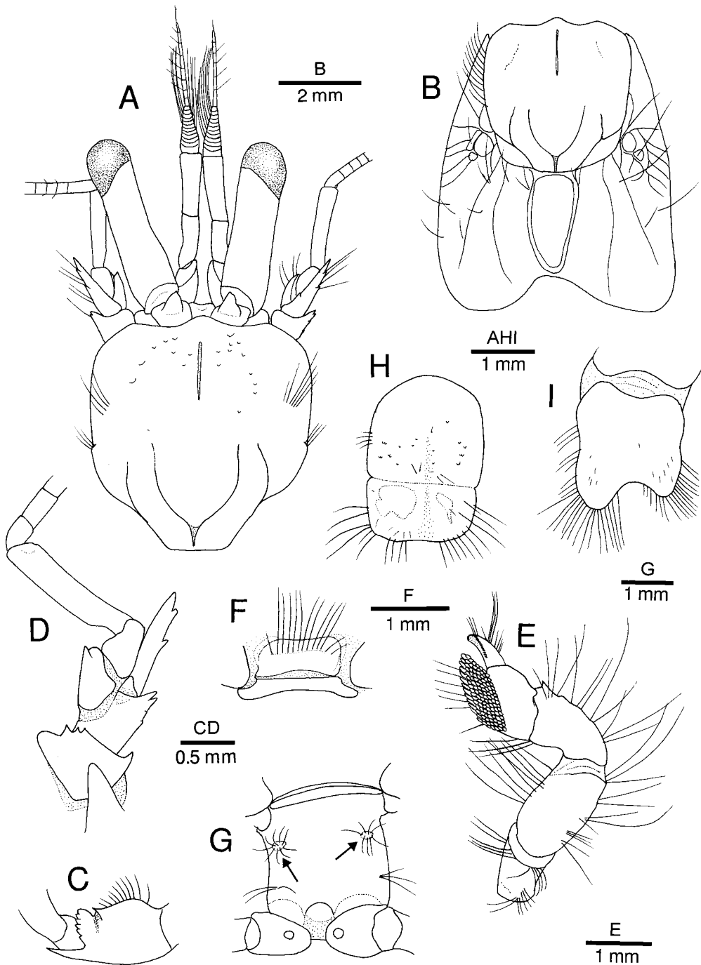
Fig. 2. Bathynarius izuensis sp. nov. Holotype male (SL 3.7 mm; NSMT-Cr S 005). A, shield and cephalic appendages, dorsal view; B, carapace, dorsal view; C, basal segment of left antennular peduncle, ventral view; D, left antennal peduncle, ventral view; E, left fourth pereopod, lateral view; F, sixth thoracic sternite, ventral view; G, seventh and eighth thoracic sternites and coxae of fifth pereopods, ventral view; H, sixth abdominal tergite, dorsal view; I, telson, dorsal view.
