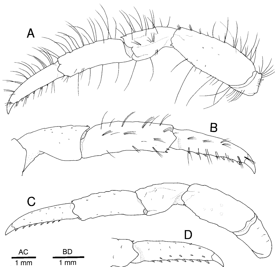
Fig. 5. Bathynarius izuensis sp. nov. Holotype male (SL 3.7 mm; NSMT-Cr S 005). A, left second pereopod, lateral view; B, same, dactylus to carpus, mesial view (setae on dorsal and ventral surfaces omitted); C, left third pereopod, lateral view (setae omitted); D, same, dactylus, mesial view (setae omitted).
