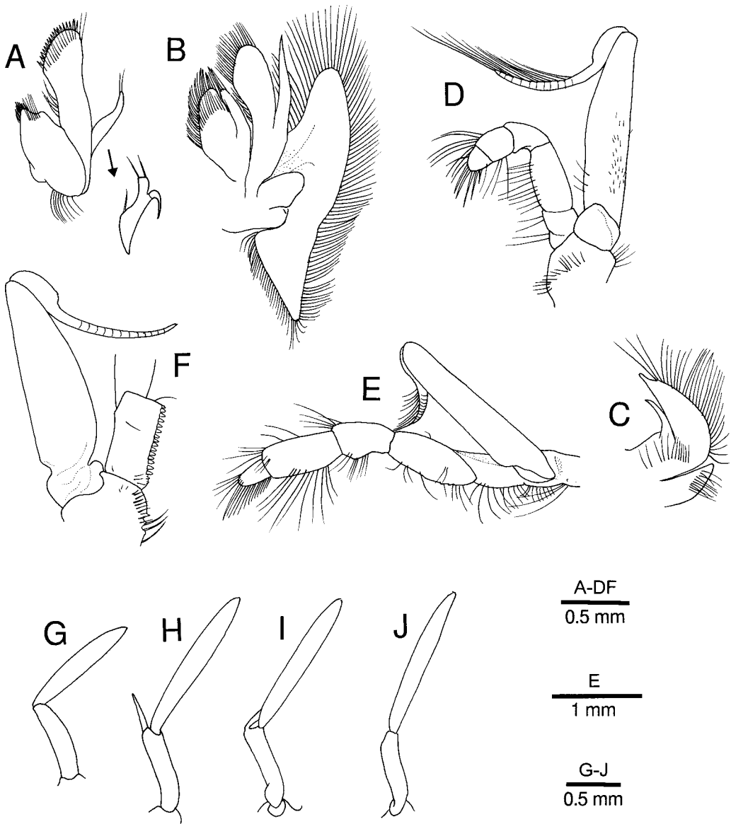
Fig. 3. Bathynarius izuensis sp. nov. Holotype male (SL 3.7 mm; NSMT-Cr S 005). Left appendages. A, maxillule, ventral view; inset, palp, lateral view; B, maxilla, ventral view; C, first maxilliped, ventral view (endites broken off; arrow indicates epipod); D, second maxilliped, ventral view; E, third maxilliped, lateral view; F, same, ischium, basis and exopod, ventral view; G, second pleopod; H, third pleopod; I, fourth pleopod; J, fifth pleopod.
