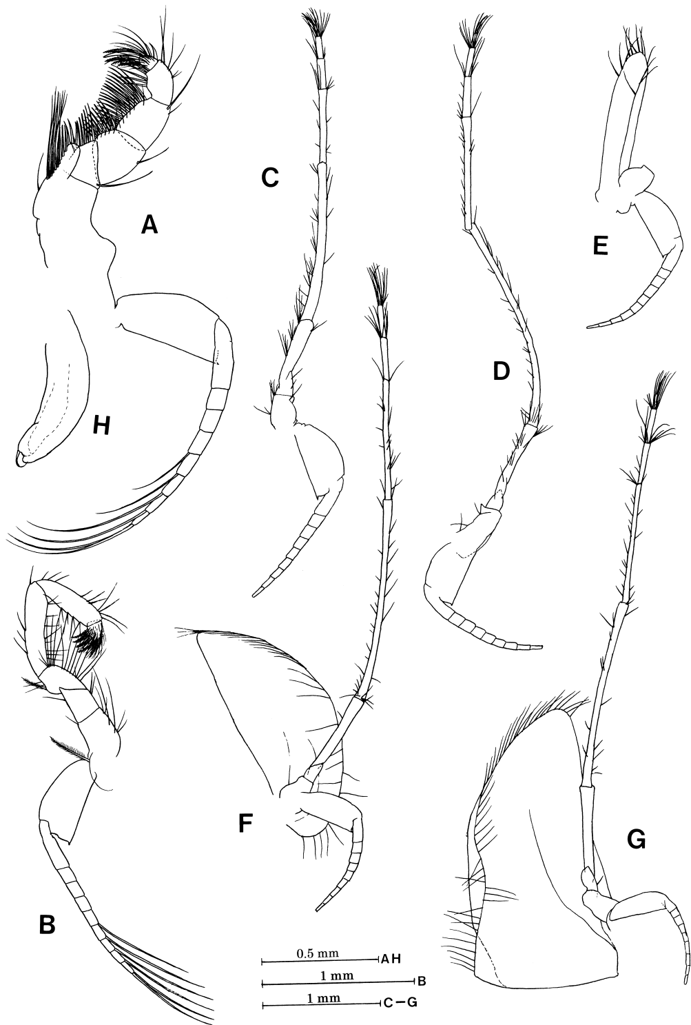
Fig. 3. Eoamblyops japonicus gen. nov., sp. nov. —A–G, holotype, female (NSMT-Cr 22391); H, one of male paratypes (8.6 mm) (NSMT-Cr 22393). A, first thoracopod; B, second thoracopod; C, third thoracopod; D, fifth thoracopod; E, exopod and oostegite of sixth thoracopod; F, seventh thoracopod; G, eighth thoracopod; H, genital organ.
