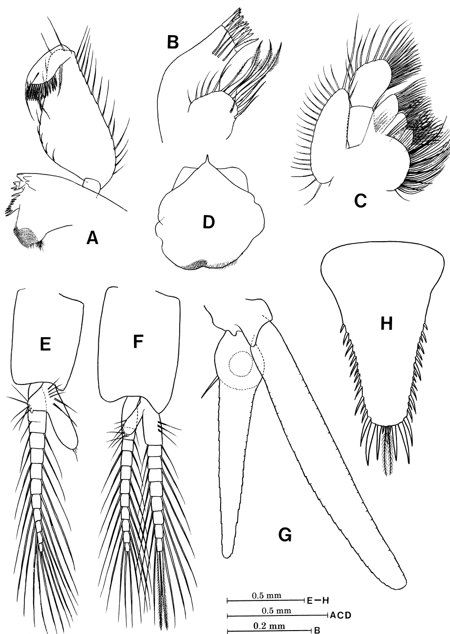
Fig. 2. Eoamblyops japonicus gen. nov., sp. nov. —A–D, G, H, holotype, female (NSMT-Cr 22391); E, F, allotype, male (NSMT-Cr 22392). A, mandible and mandibular palp; B, maxillule; C, maxilla; D, labrum; E, first pleopod; F, fourth pleopod; G, uropod; H, telson.
